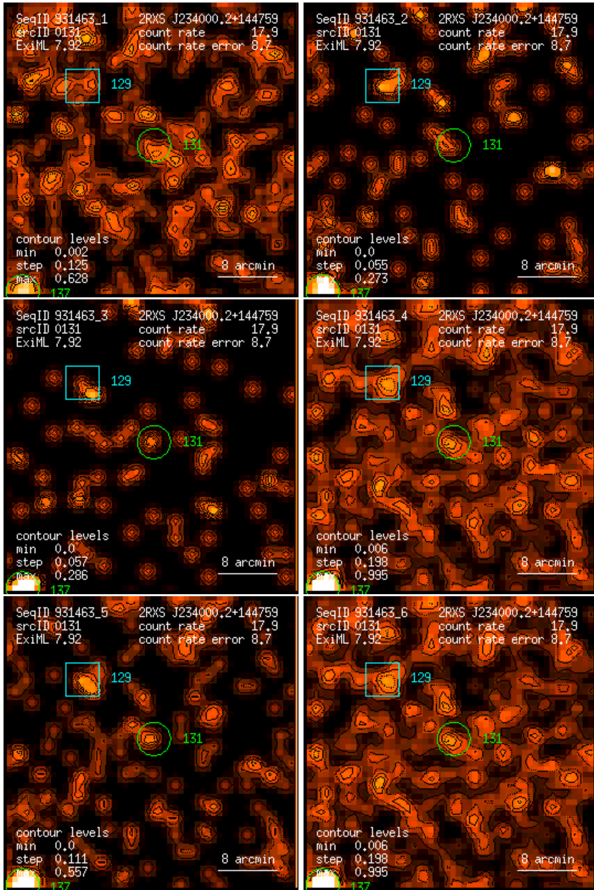
Figure 131: RASS 931463: detection 0131: band rate images, Gaussian filter: (1) PSPC channels 11 – 41, (2) 52 – 90, (3) 91 – 201, (4) 11 – 235, (5) 52 – 201, (6) 11 – 201. Broad band rates in counts/ks. Band rate contour levels in counts/ks/arcmin 2 .
