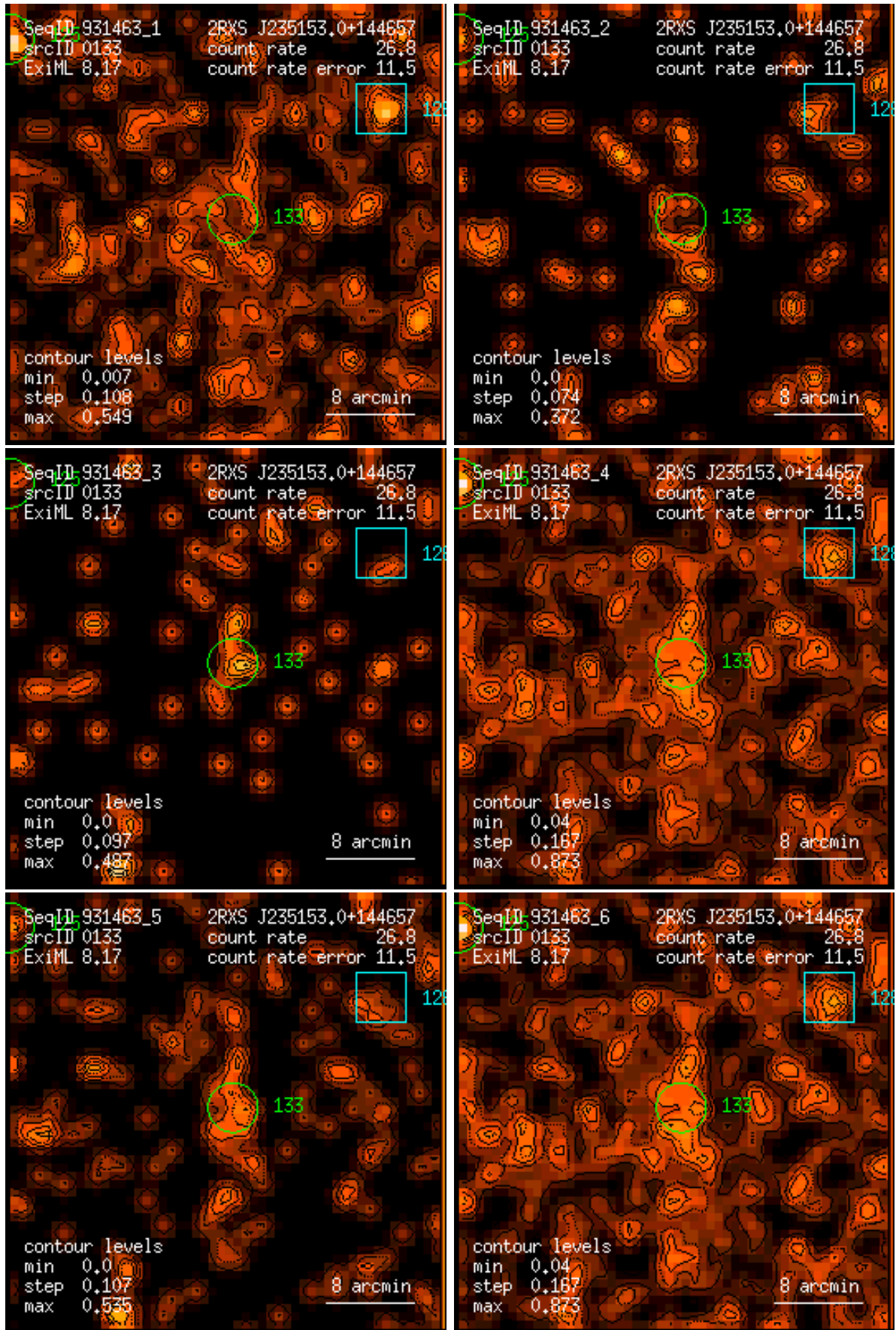
Figure 133: RASS 931463: detection 0133: band rate images, Gaussian filter: (1) PSPC channels 11 – 41, (2) 52 – 90, (3) 91 – 201, (4) 11 – 235, (5) 52 – 201, (6) 11 – 201. Broad band rates in counts/ks. Band rate contour levels in counts/ks/arcmin 2 .
