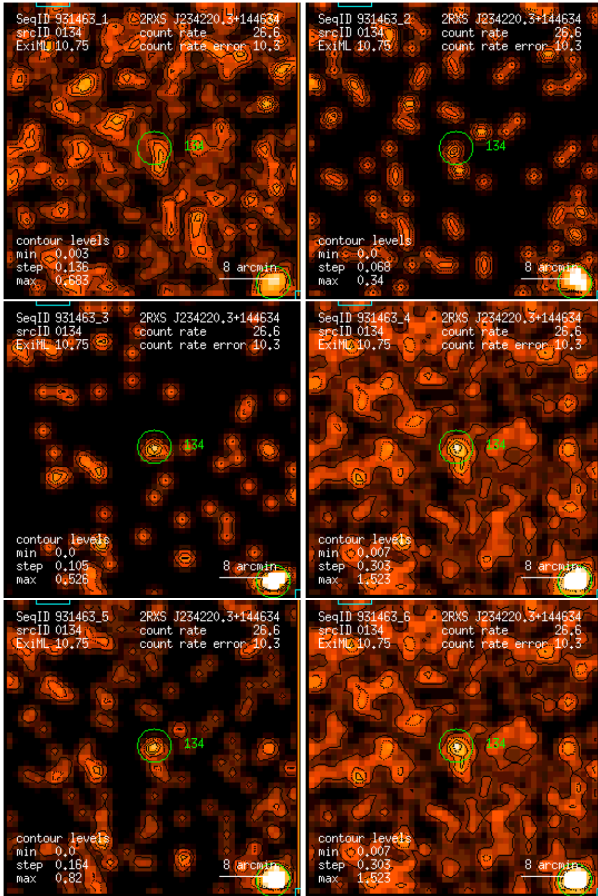
Figure 134: RASS 931463: detection 0134: band rate images, Gaussian filter: (1) PSPC channels 11 – 41, (2) 52 – 90, (3) 91 – 201, (4) 11 – 235, (5) 52 – 201, (6) 11 – 201. Broad band rates in counts/ks. Band rate contour levels in counts/ks/arcmin 2 .
