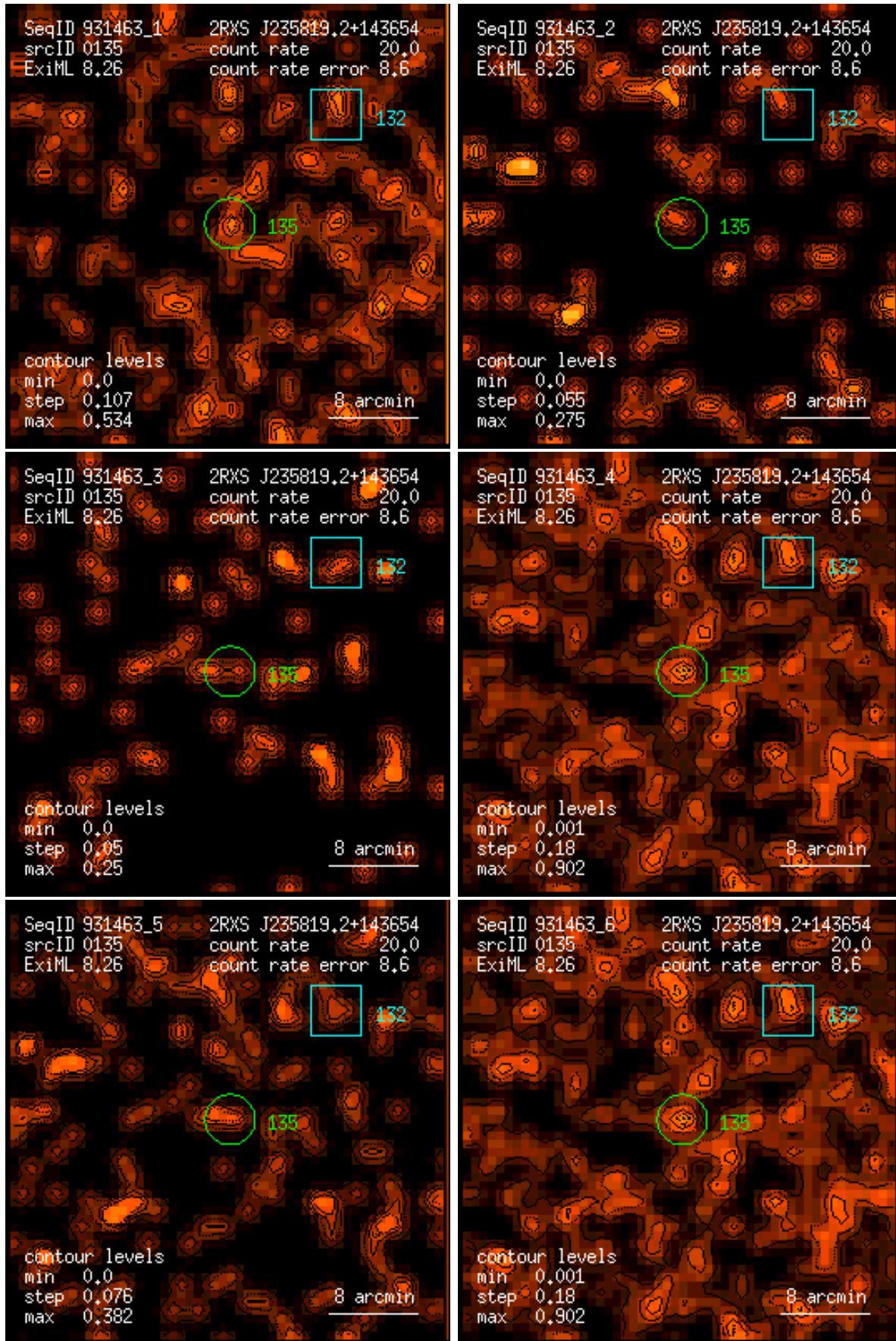
Figure 135: RASS 931463: detection 0135: band rate images, Gaussian filter: (1) PSPC channels 11 – 41, (2) 52 – 90, (3) 91 – 201, (4) 11 – 235, (5) 52 – 201, (6) 11 – 201. Broad band rates in counts/ks. Band rate contour levels in counts/ks/arcmin 2 .
