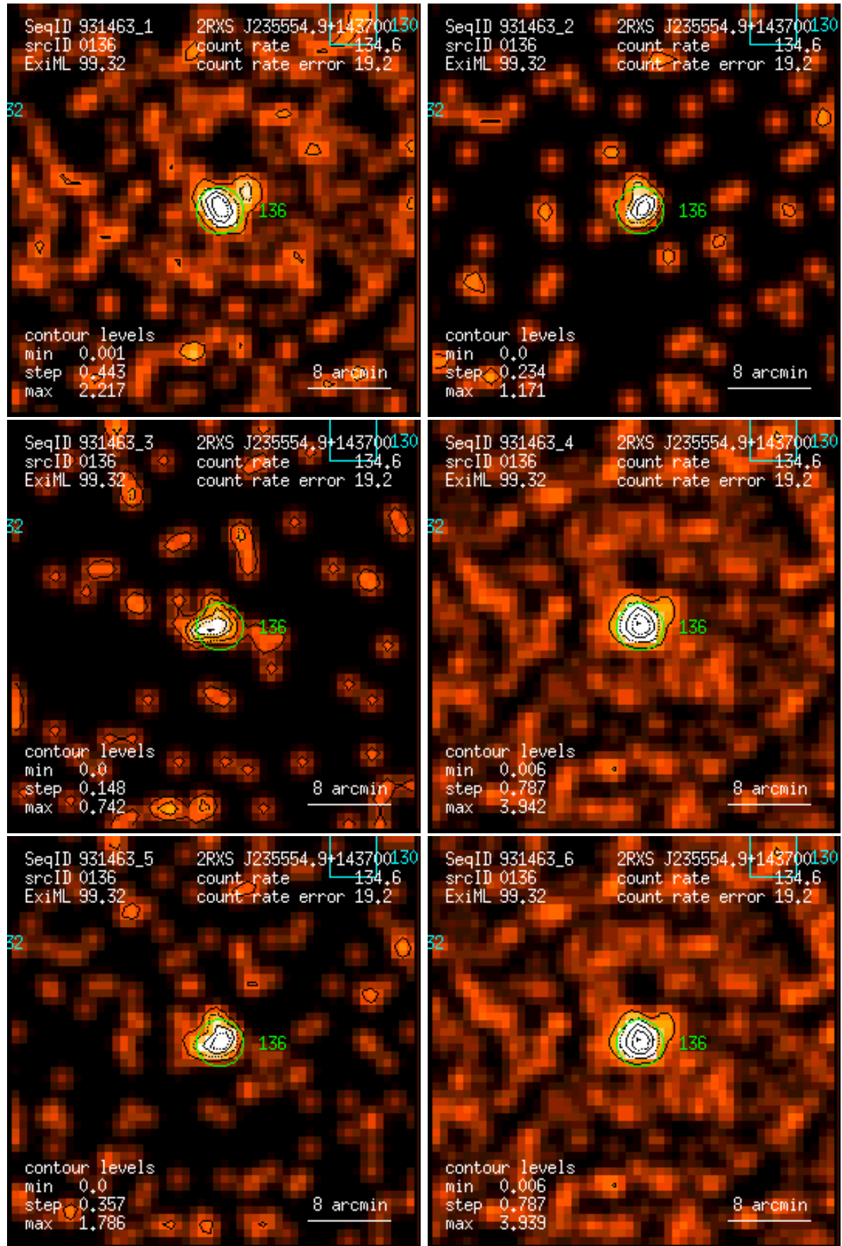
Figure 136: RASS 931463: detection 0136: band rate images, Gaussian filter: (1) PSPC channels 11 – 41, (2) 52 – 90, (3) 91 – 201, (4) 11 – 235, (5) 52 – 201, (6) 11 – 201. Broad band rates in counts/ks. Band rate contour levels in counts/ks/arcmin 2 .
