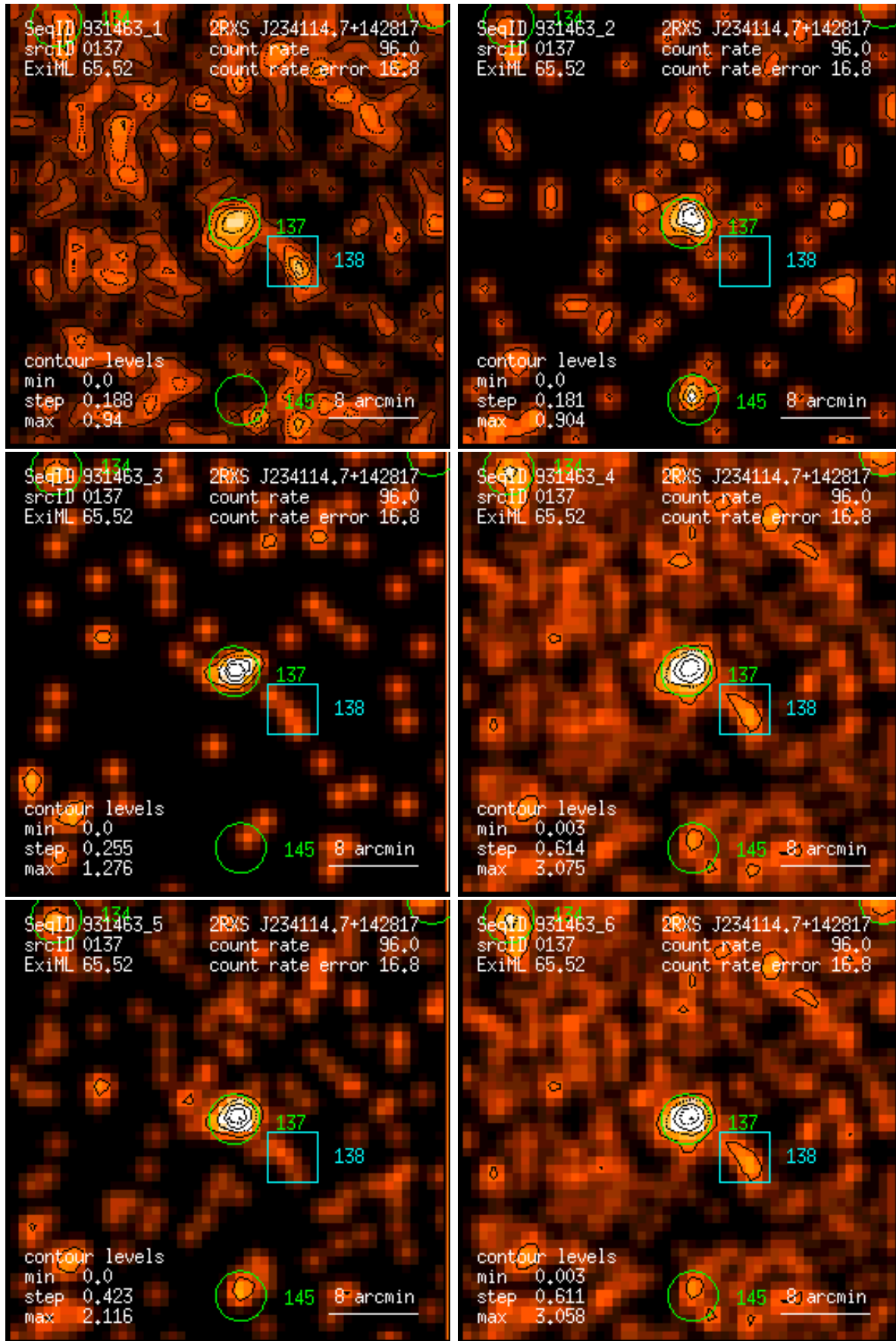
Figure 137: RASS 931463: detection 0137: band rate images, Gaussian filter: (1) PSPC channels 11 – 41, (2) 52 – 90, (3) 91 – 201, (4) 11 – 235, (5) 52 – 201, (6) 11 – 201. Broad band rates in counts/ks. Band rate contour levels in counts/ks/arcmin 2 .
