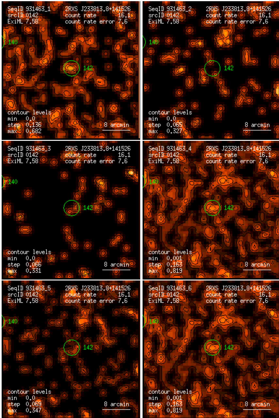
Figure 142: RASS 931463: detection 0142: band rate images, Gaussian filter: (1) PSPC channels 11 – 41, (2) 52 – 90, (3) 91 – 201, (4) 11 – 235, (5) 52 – 201, (6) 11 – 201. Broad band rates in counts/ks. Band rate contour levels in counts/ks/arcmin 2 .
