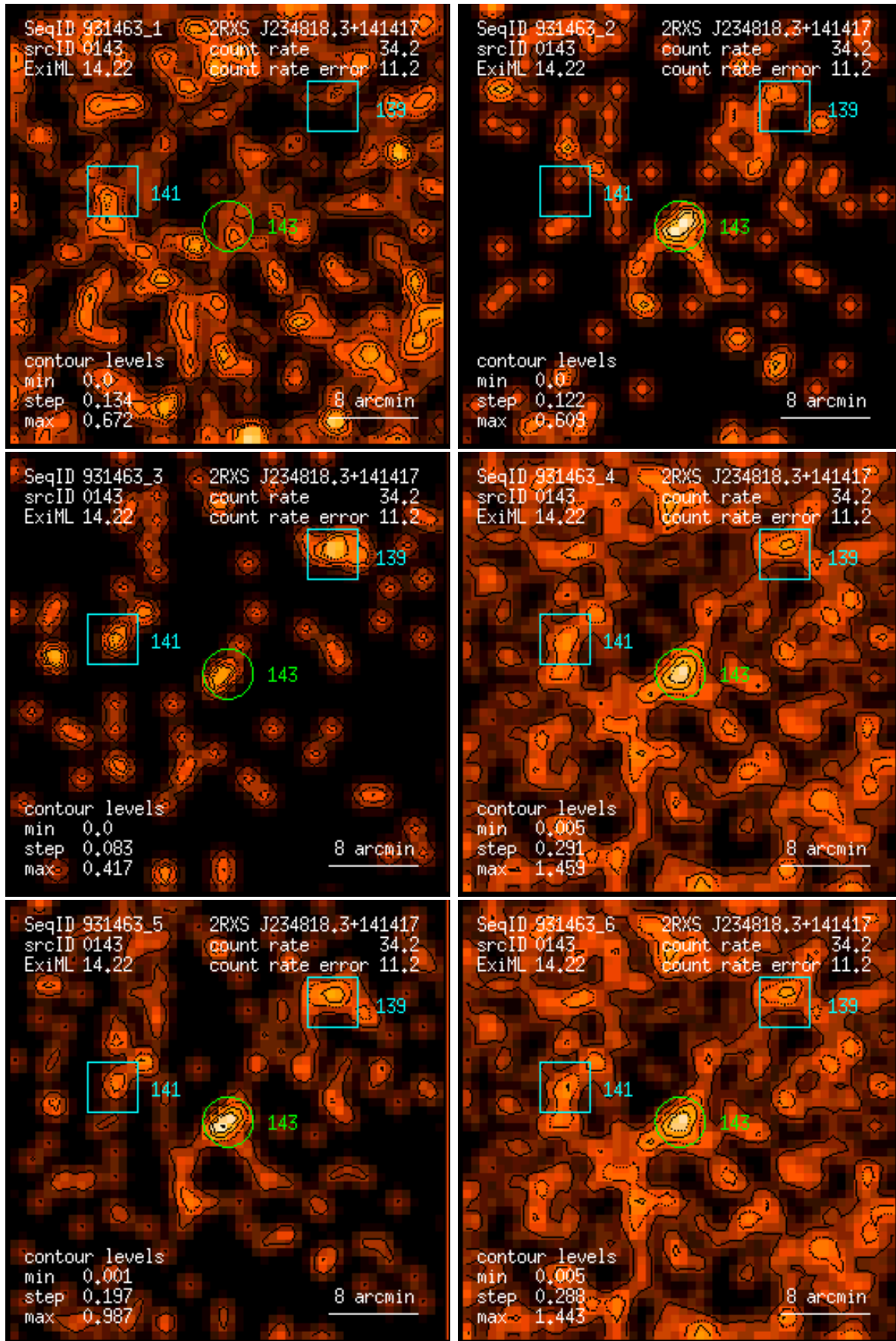
Figure 143: RASS 931463: detection 0143: band rate images, Gaussian filter: (1) PSPC channels 11 – 41, (2) 52 – 90, (3) 91 – 201, (4) 11 – 235, (5) 52 – 201, (6) 11 – 201. Broad band rates in counts/ks. Band rate contour levels in counts/ks/arcmin 2 .
