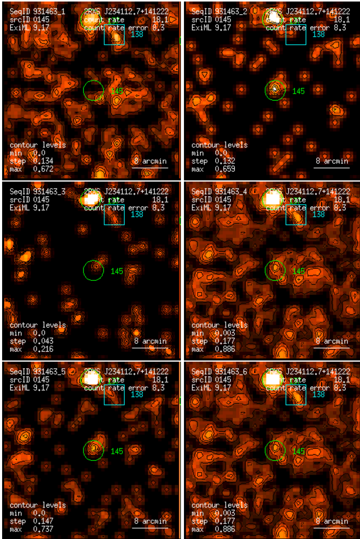
Figure 145: RASS 931463: detection 0145: band rate images, Gaussian filter: (1) PSPC channels 11 – 41, (2) 52 – 90, (3) 91 – 201, (4) 11 – 235, (5) 52 – 201, (6) 11 – 201. Broad band rates in counts/ks. Band rate contour levels in counts/ks/arcmin 2 .
