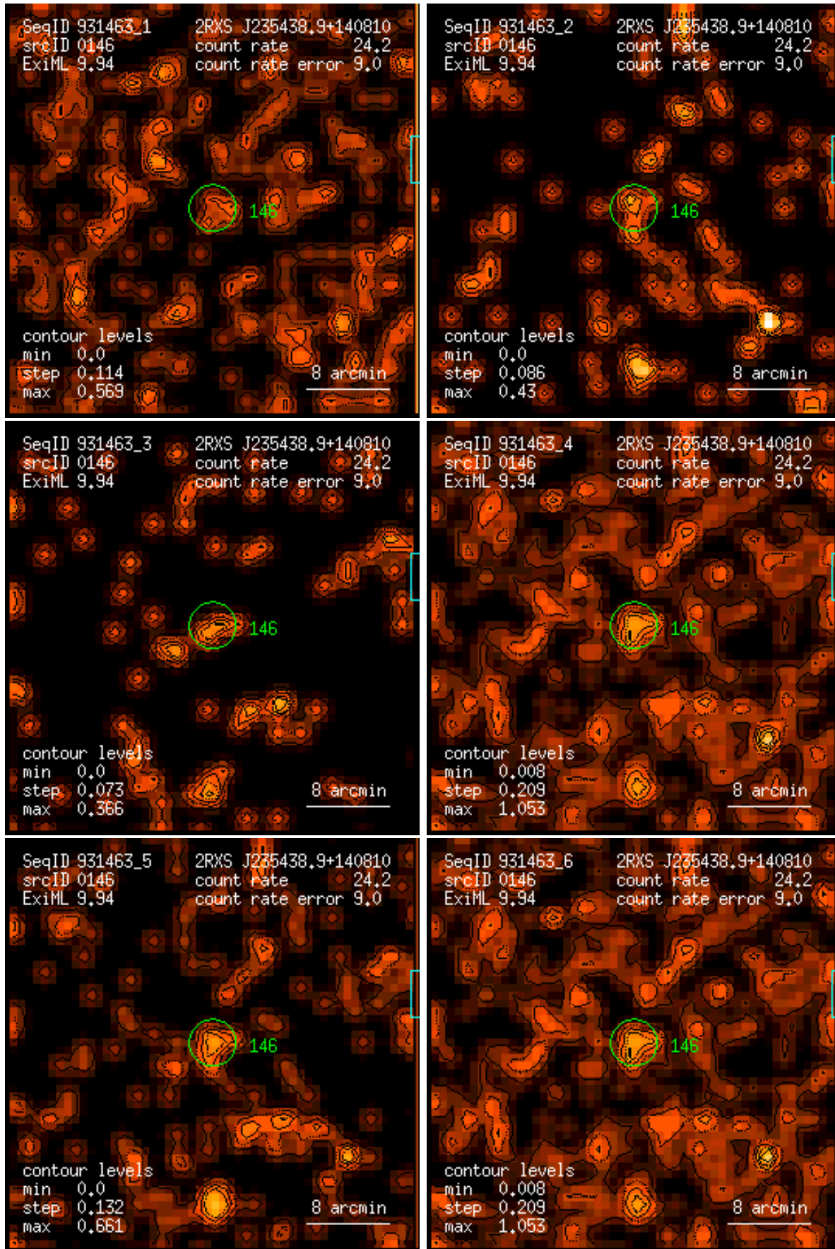
Figure 146: RASS 931463: detection 0146: band rate images, Gaussian filter: (1) PSPC channels 11 – 41, (2) 52 – 90, (3) 91 – 201, (4) 11 – 235, (5) 52 – 201, (6) 11 – 201. Broad band rates in counts/ks. Band rate contour levels in counts/ks/arcmin 2 .
