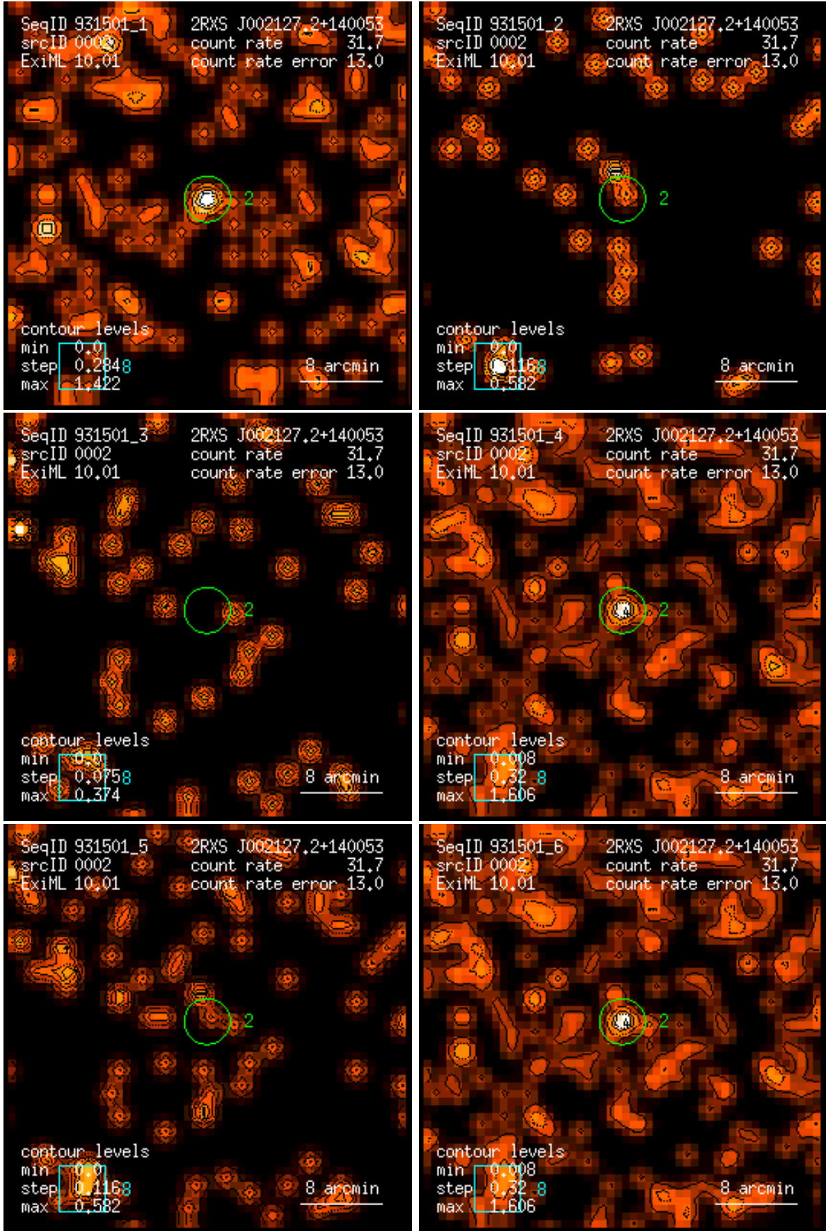
Figure 2: RASS 931501: detection 0002: band rate images, Gaussian filter: (1) PSPC channels 11 – 41, (2) 52 – 90, (3) 91 – 201, (4) 11 – 235, (5) 52 – 201, (6) 11 – 201. Broad band rates in counts/ks. Band rate contour levels in counts/ks/arcmin 2 .
