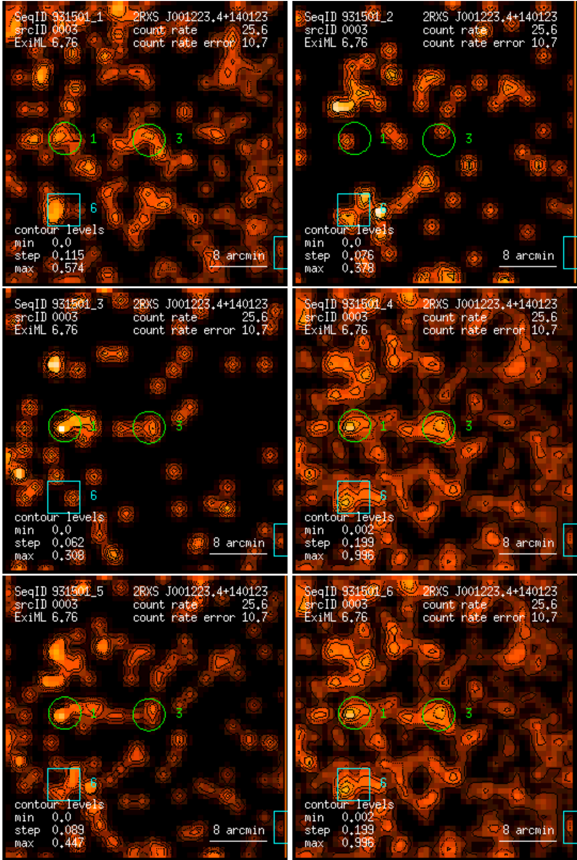
Figure 3: RASS 931501: detection 0003: band rate images, Gaussian filter: (1) PSPC channels 11 – 41, (2) 52 – 90, (3) 91 – 201, (4) 11 – 235, (5) 52 – 201, (6) 11 – 201. Broad band rates in counts/ks. Band rate contour levels in counts/ks/arcmin 2 .
