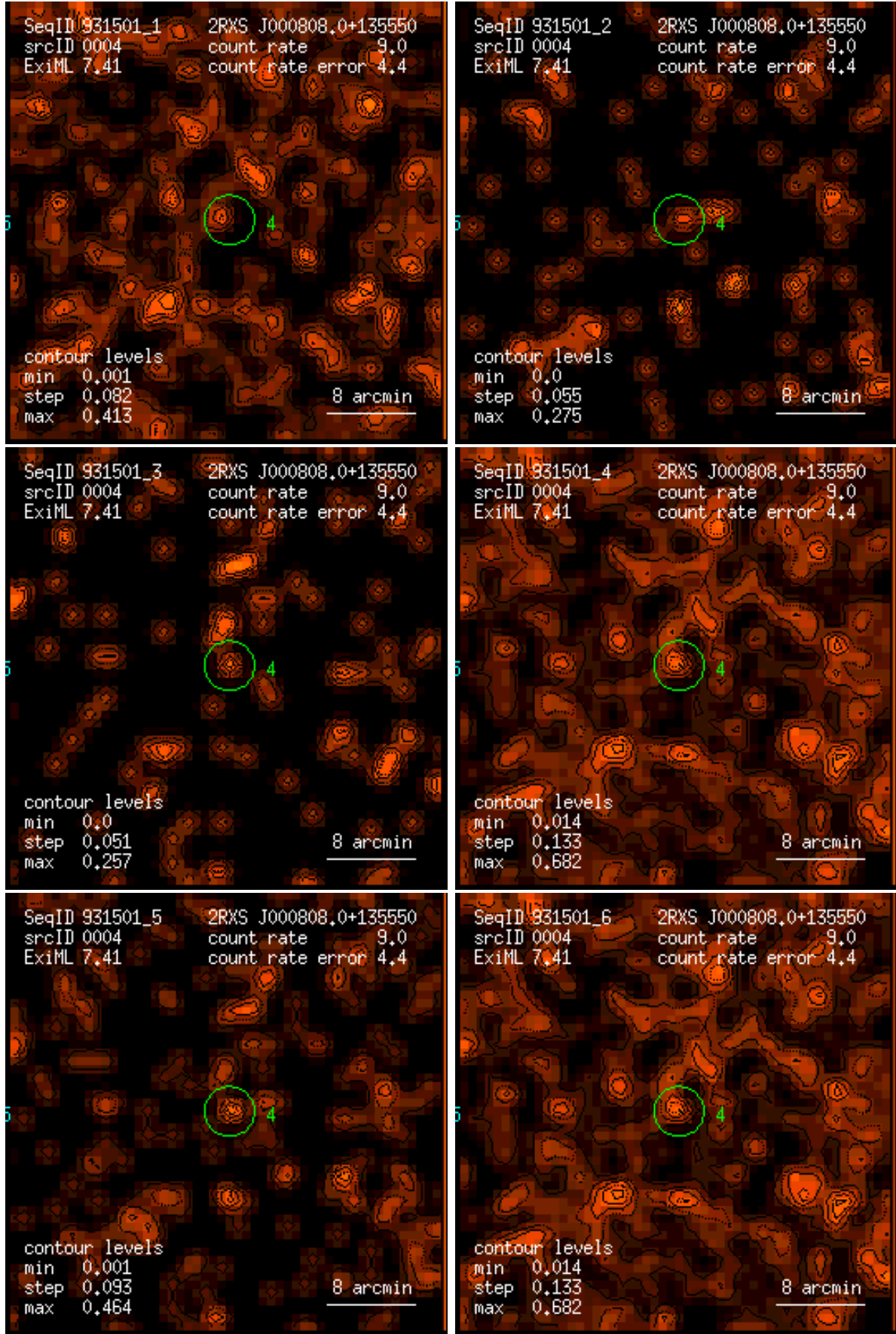
Figure 4: RASS 931501: detection 0004: band rate images, Gaussian filter: (1) PSPC channels 11 – 41, (2) 52 – 90, (3) 91 – 201, (4) 11 – 235, (5) 52 – 201, (6) 11 – 201. Broad band rates in counts/ks. Band rate contour levels in counts/ks/arcmin 2 .
