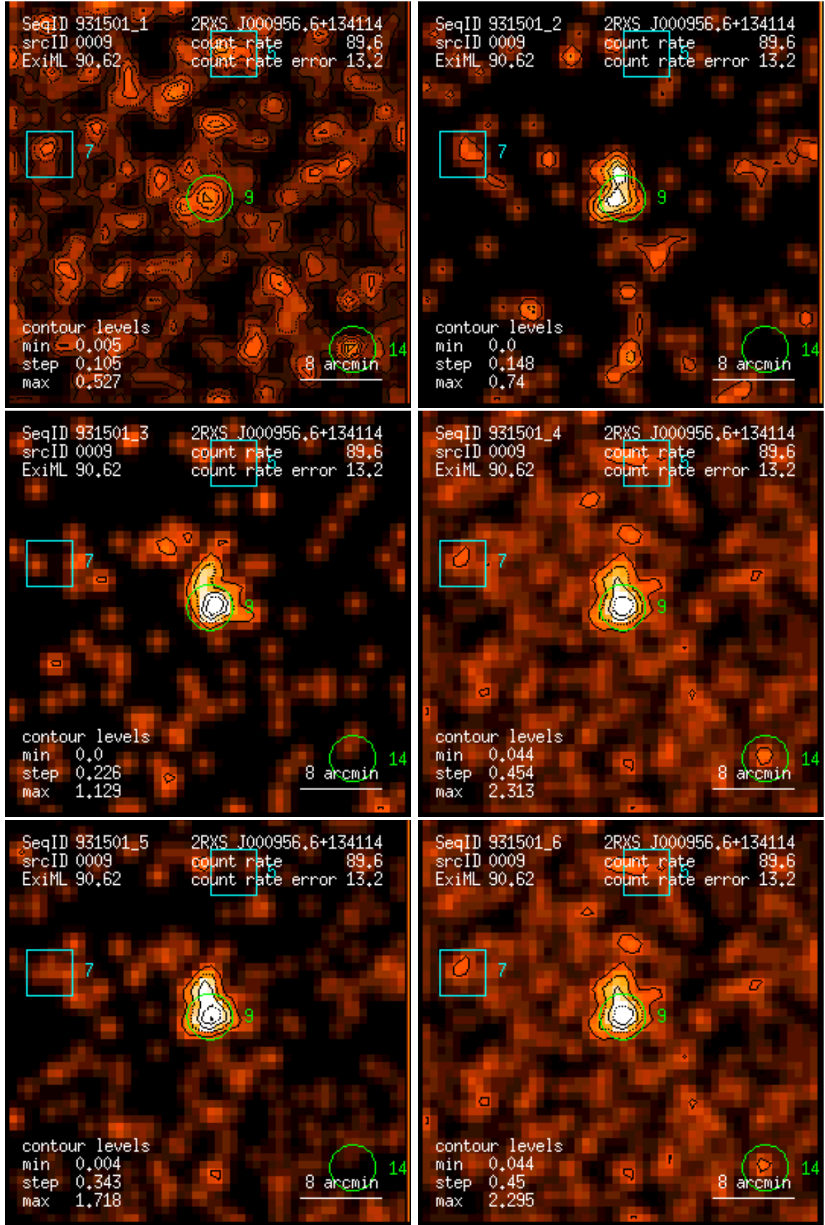
Figure 9: RASS 931501: detection 0009: band rate images, Gaussian filter: (1) PSPC channels 11 – 41, (2) 52 – 90, (3) 91 – 201, (4) 11 – 235, (5) 52 – 201, (6) 11 – 201. Broad band rates in counts/ks. Band rate contour levels in counts/ks/arcmin 2 .
