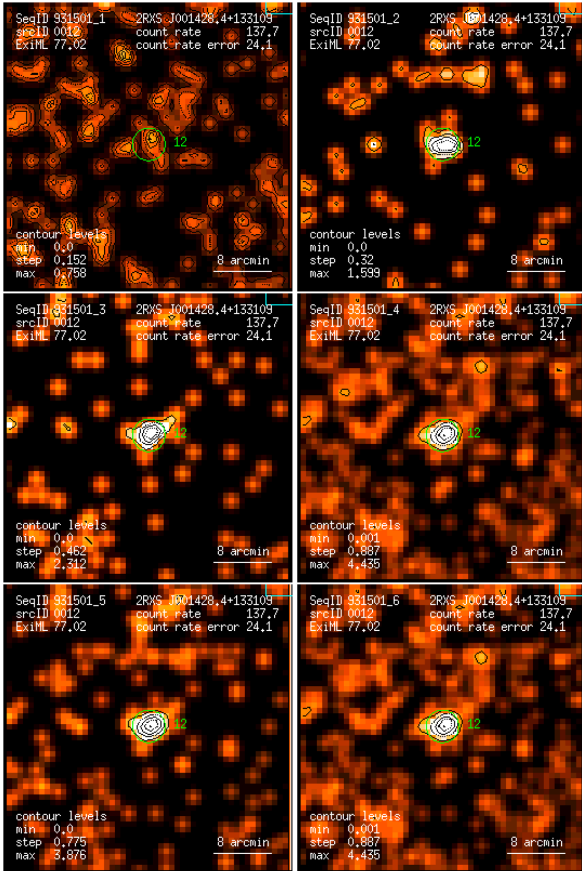
Figure 12: RASS 931501: detection 0012: band rate images, Gaussian filter: (1) PSPC channels 11 – 41, (2) 52 – 90, (3) 91 – 201, (4) 11 – 235, (5) 52 – 201, (6) 11 – 201. Broad band rates in counts/ks. Band rate contour levels in counts/ks/arcmin 2 .
