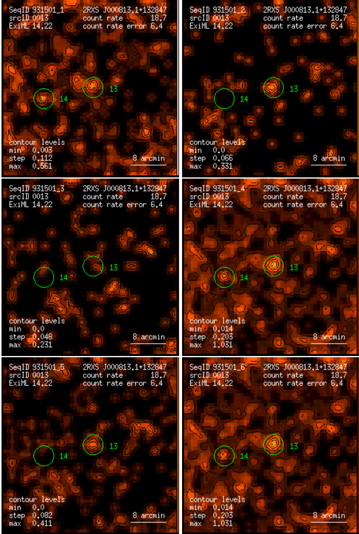
Figure 13: RASS 931501: detection 0013: band rate images, Gaussian filter: (1) PSPC channels 11 – 41, (2) 52 – 90, (3) 91 – 201, (4) 11 – 235, (5) 52 – 201, (6) 11 – 201. Broad band rates in counts/ks. Band rate contour levels in counts/ks/arcmin 2 .
