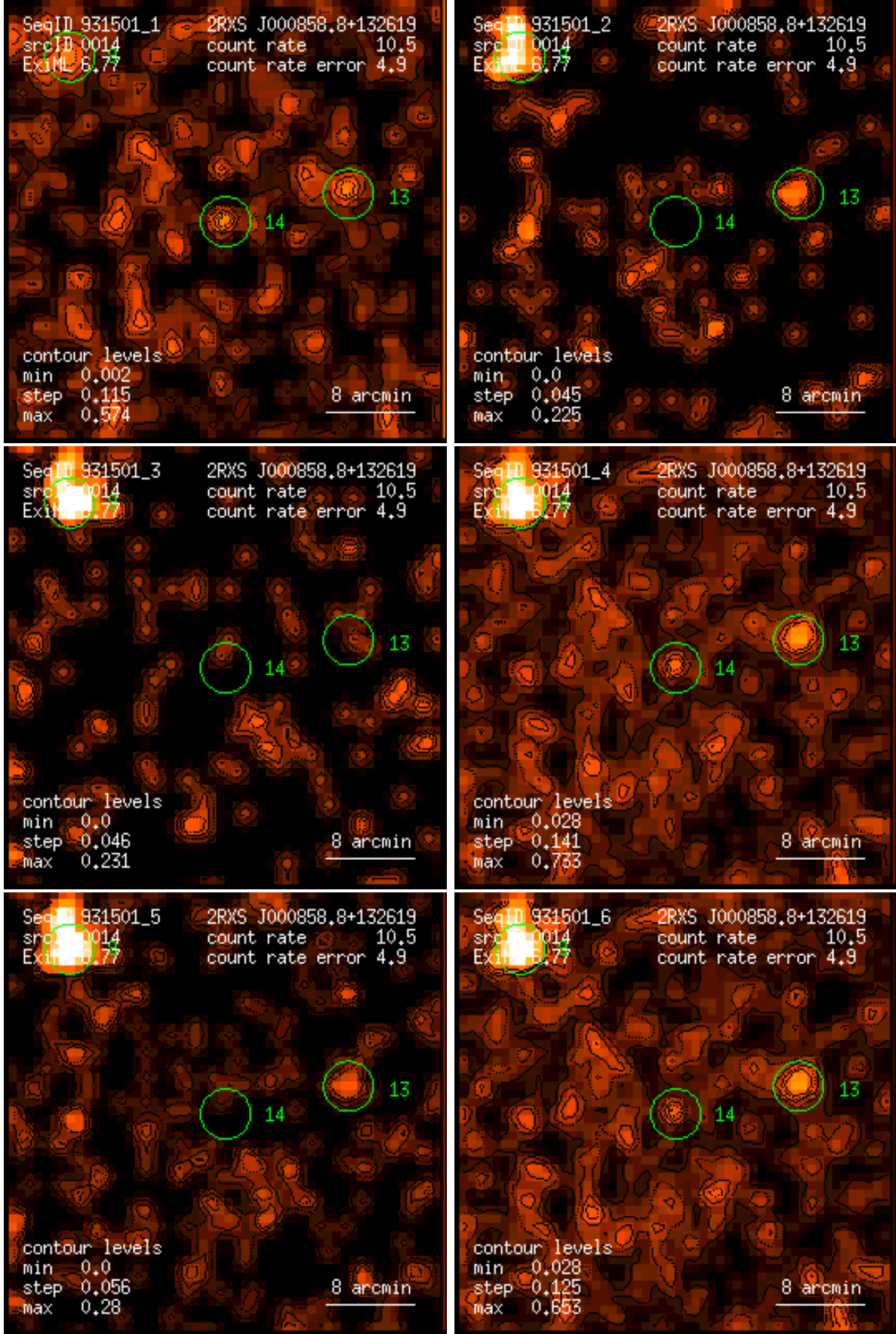
Figure 14: RASS 931501: detection 0014: band rate images, Gaussian filter: (1) PSPC channels 11 – 41, (2) 52 – 90, (3) 91 – 201, (4) 11 – 235, (5) 52 – 201, (6) 11 – 201. Broad band rates in counts/ks. Band rate contour levels in counts/ks/arcmin 2 .
