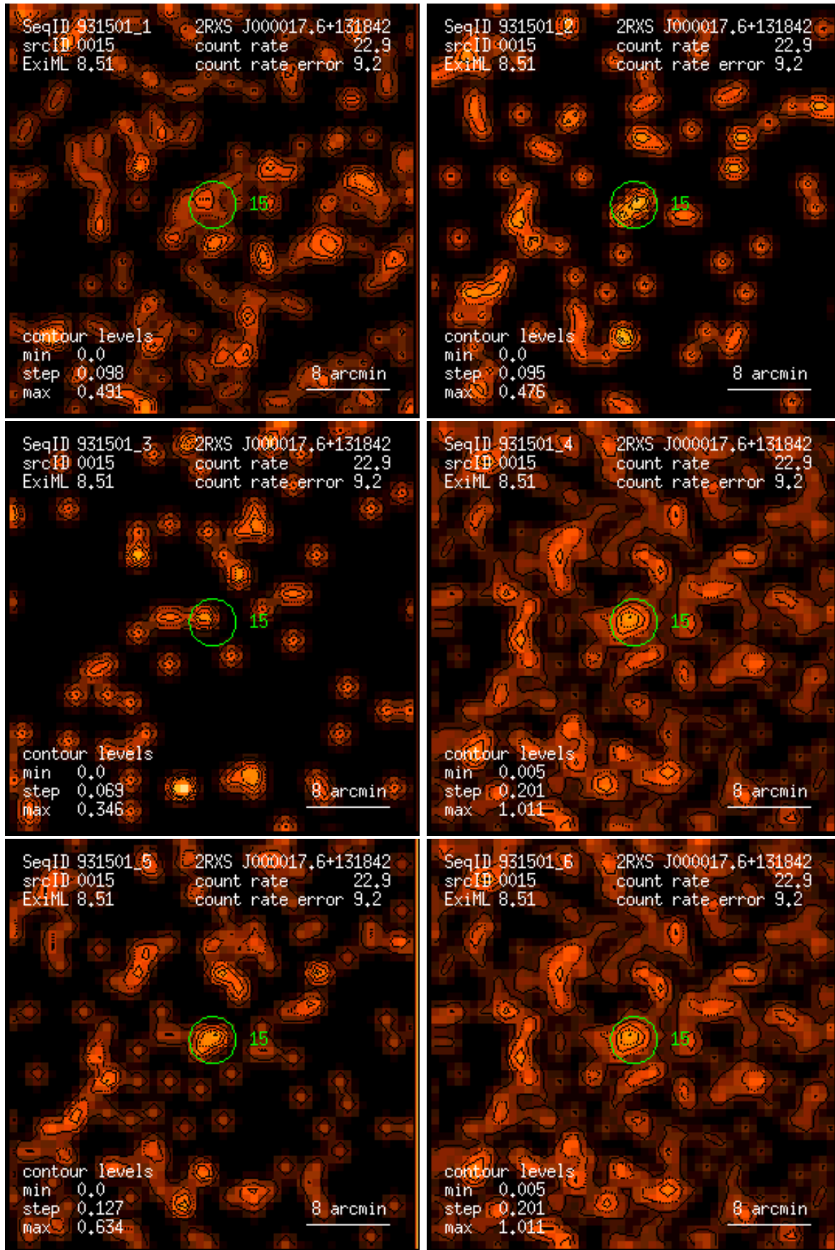
Figure 15: RASS 931501: detection 0015: band rate images, Gaussian filter: (1) PSPC channels 11 – 41, (2) 52 – 90, (3) 91 – 201, (4) 11 – 235, (5) 52 – 201, (6) 11 – 201. Broad band rates in counts/ks. Band rate contour levels in counts/ks/arcmin 2 .
