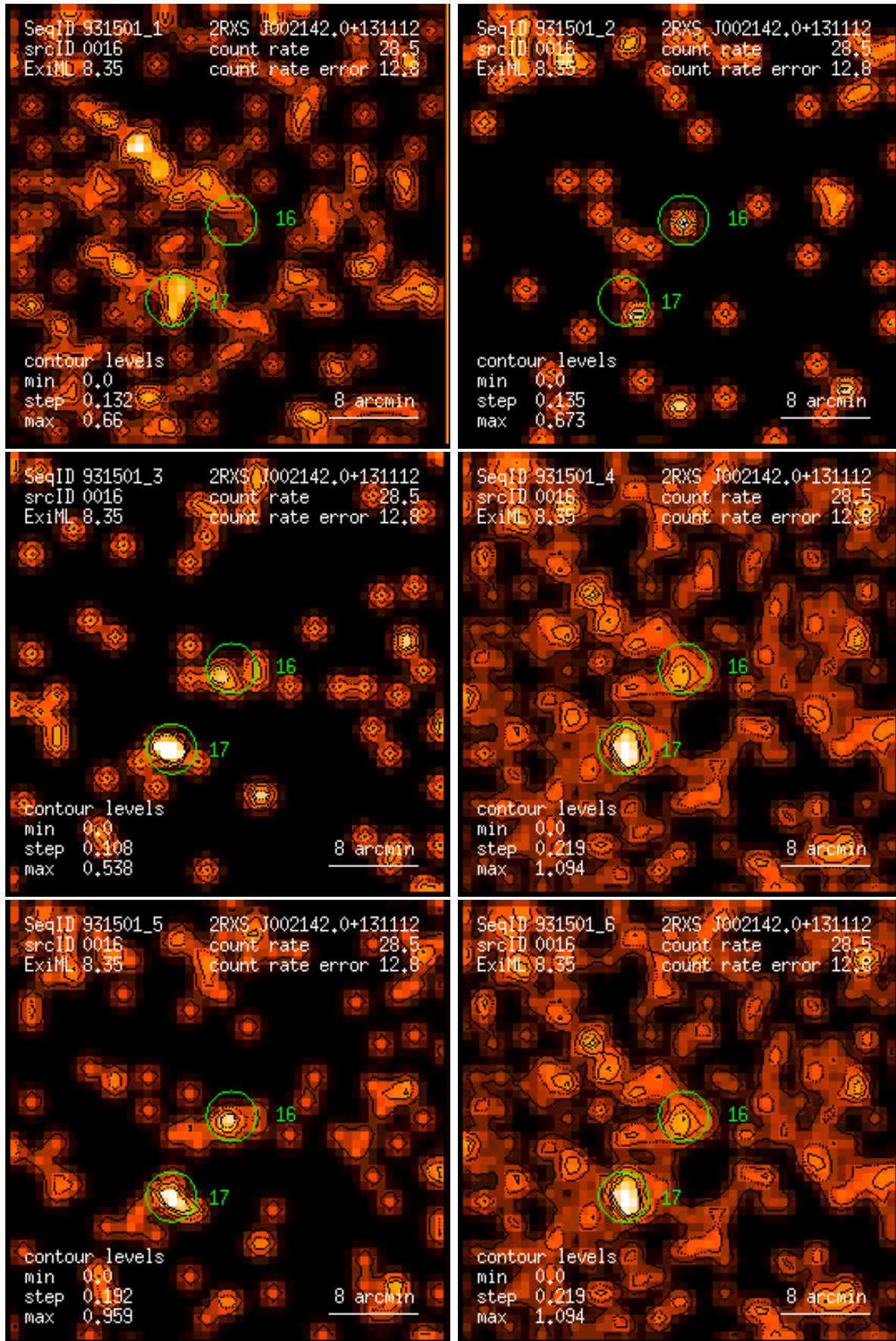
Figure 16: RASS 931501: detection 0016: band rate images, Gaussian filter: (1) PSPC channels 11 – 41, (2) 52 – 90, (3) 91 – 201, (4) 11 – 235, (5) 52 – 201, (6) 11 – 201. Broad band rates in counts/ks. Band rate contour levels in counts/ks/arcmin 2 .
