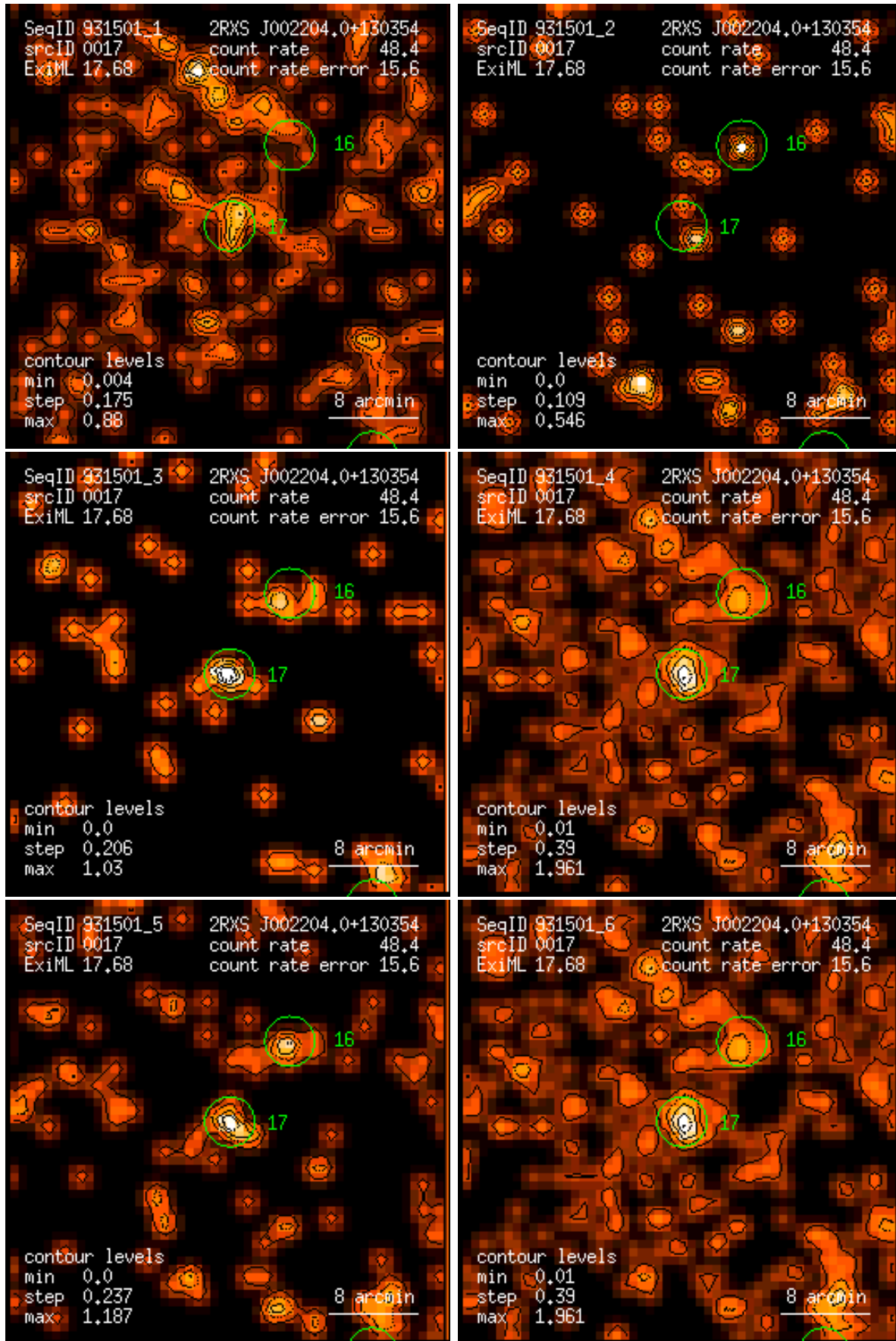
Figure 17: RASS 931501: detection 0017: band rate images, Gaussian filter: (1) PSPC channels 11 – 41, (2) 52 – 90, (3) 91 – 201, (4) 11 – 235, (5) 52 – 201, (6) 11 – 201. Broad band rates in counts/ks. Band rate contour levels in counts/ks/arcmin 2 .
