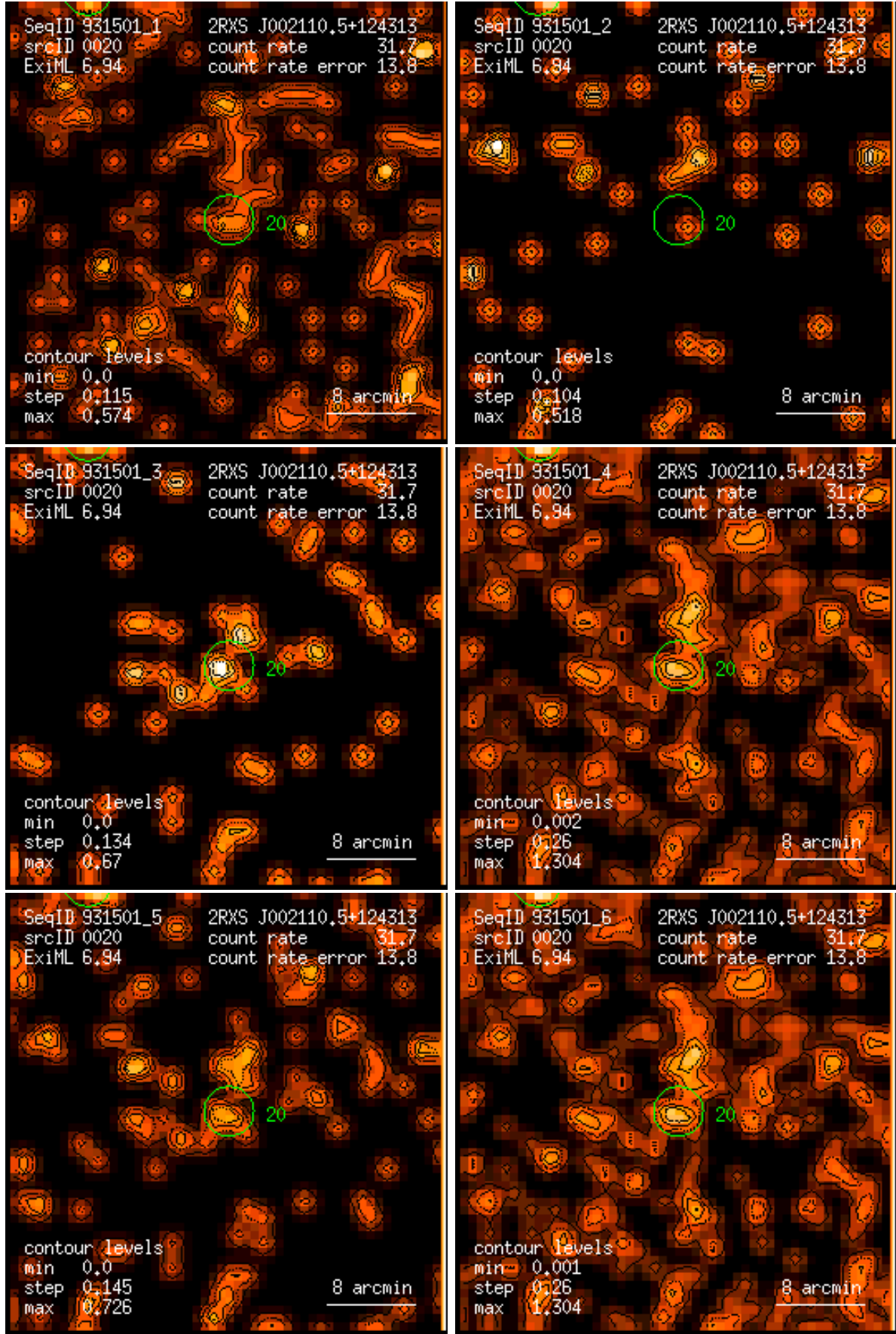
Figure 20: RASS 931501: detection 0020: band rate images, Gaussian filter: (1) PSPC channels 11 – 41, (2) 52 – 90, (3) 91 – 201, (4) 11 – 235, (5) 52 – 201, (6) 11 – 201. Broad band rates in counts/ks. Band rate contour levels in counts/ks/arcmin 2 .
