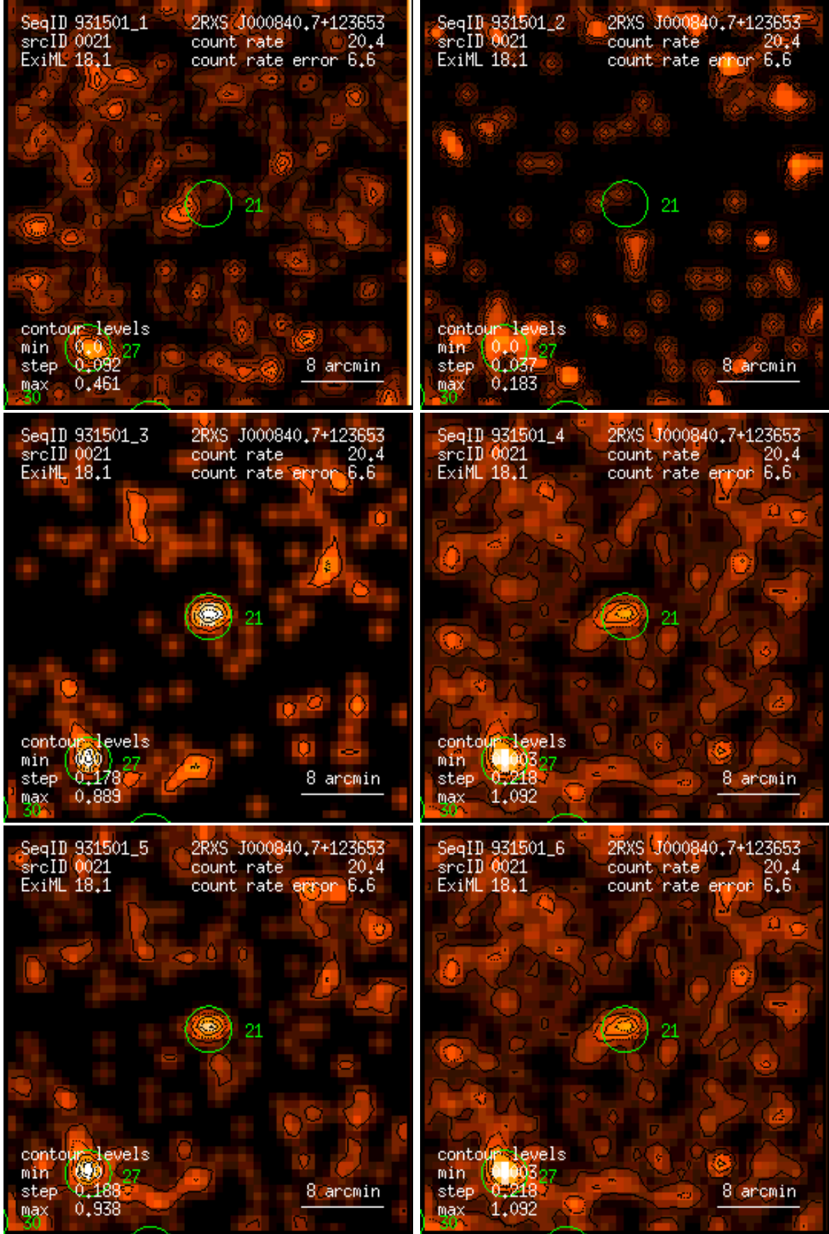
Figure 21: RASS 931501: detection 0021: band rate images, Gaussian filter: (1) PSPC channels 11 – 41, (2) 52 – 90, (3) 91 – 201, (4) 11 – 235, (5) 52 – 201, (6) 11 – 201. Broad band rates in counts/ks. Band rate contour levels in counts/ks/arcmin 2 .
