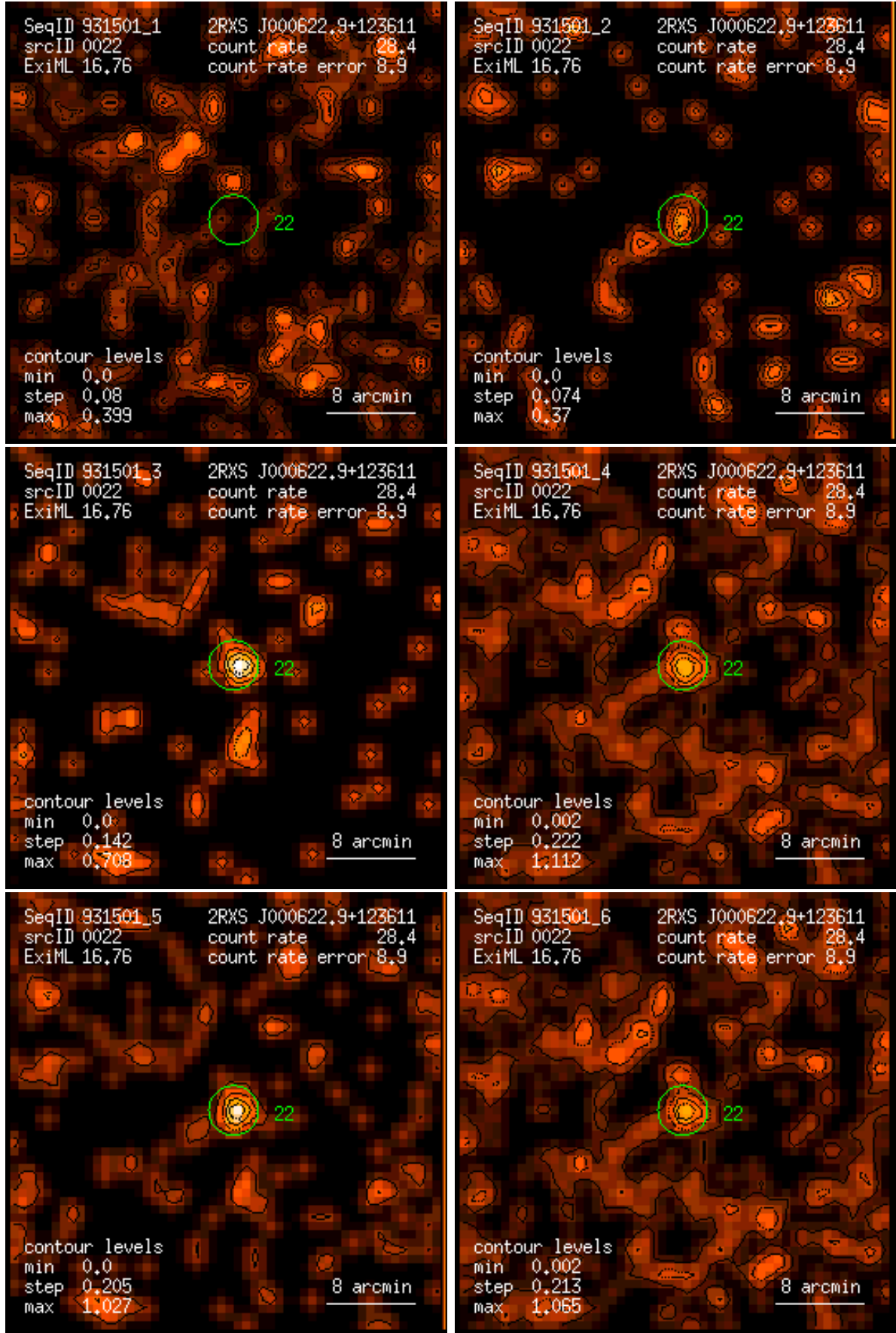
Figure 22: RASS 931501: detection 0022: band rate images, Gaussian filter: (1) PSPC channels 11 – 41, (2) 52 – 90, (3) 91 – 201, (4) 11 – 235, (5) 52 – 201, (6) 11 – 201. Broad band rates in counts/ks. Band rate contour levels in counts/ks/arcmin 2 .
