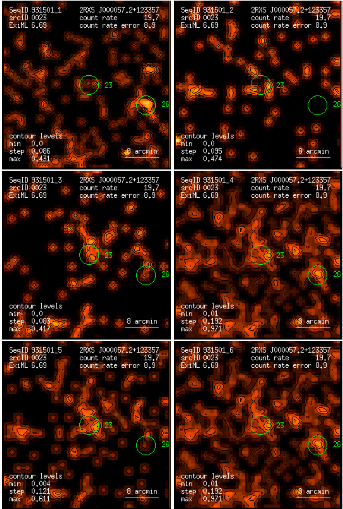
Figure 23: RASS 931501: detection 0023: band rate images, Gaussian filter: (1) PSPC channels 11 – 41, (2) 52 – 90, (3) 91 – 201, (4) 11 – 235, (5) 52 – 201, (6) 11 – 201. Broad band rates in counts/ks. Band rate contour levels in counts/ks/arcmin 2 .
