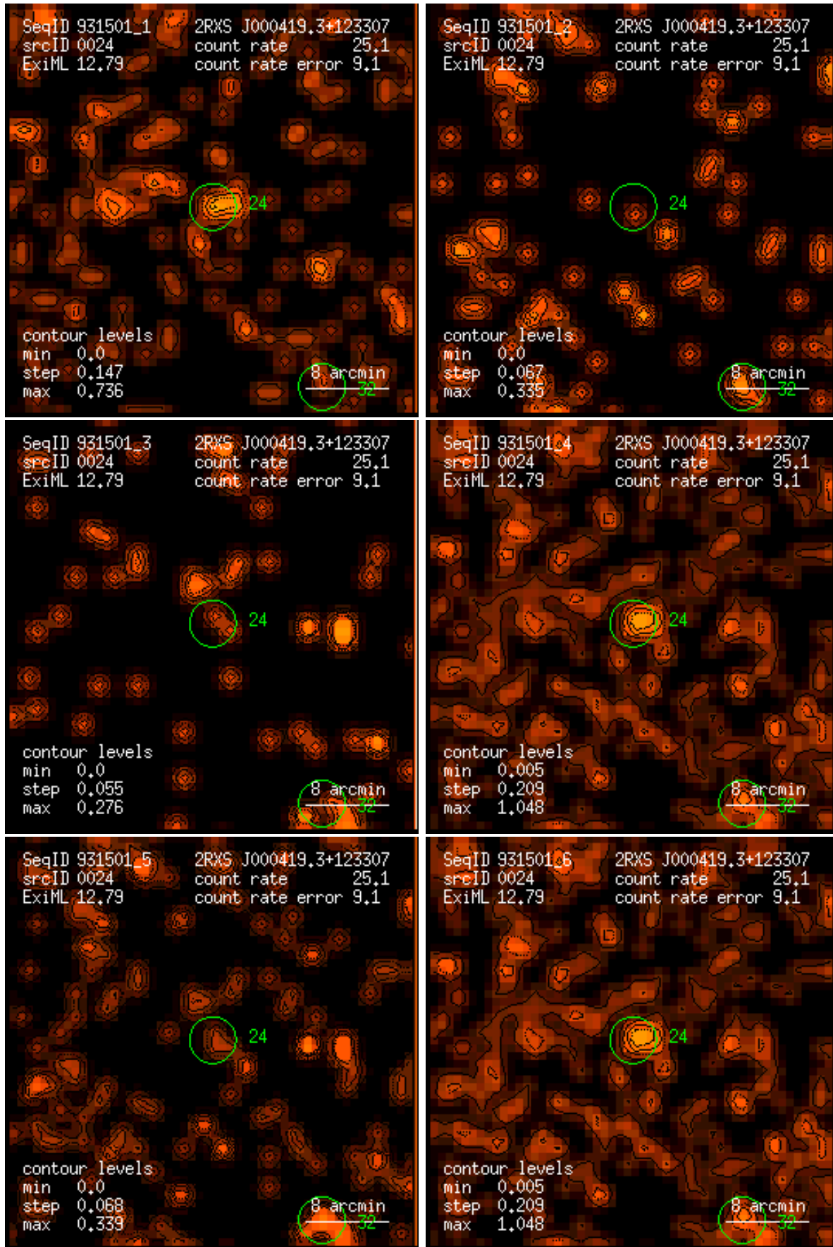
Figure 24: RASS 931501: detection 0024: band rate images, Gaussian filter: (1) PSPC channels 11 – 41, (2) 52 – 90, (3) 91 – 201, (4) 11 – 235, (5) 52 – 201, (6) 11 – 201. Broad band rates in counts/ks. Band rate contour levels in counts/ks/arcmin 2 .
