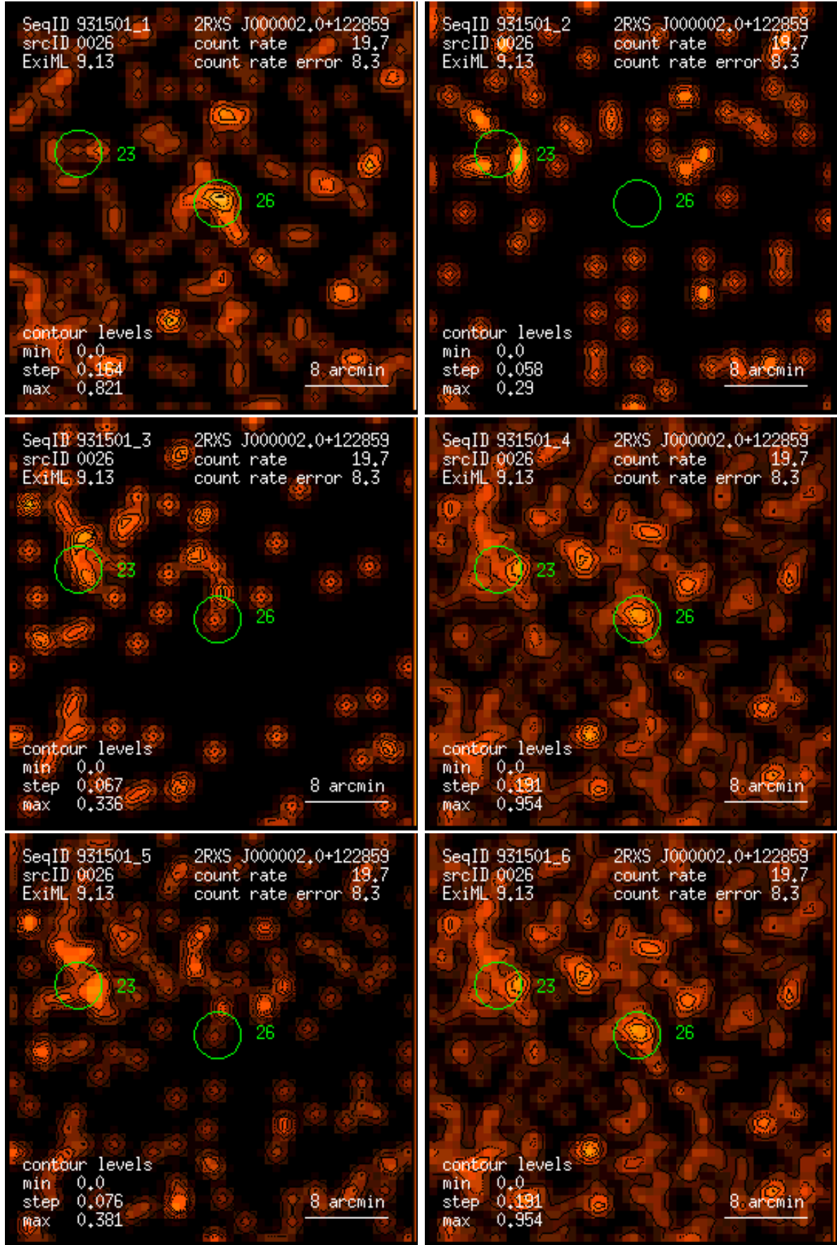
Figure 26: RASS 931501: detection 0026: band rate images, Gaussian filter: (1) PSPC channels 11 – 41, (2) 52 – 90, (3) 91 – 201, (4) 11 – 235, (5) 52 – 201, (6) 11 – 201. Broad band rates in counts/ks. Band rate contour levels in counts/ks/arcmin 2 .
