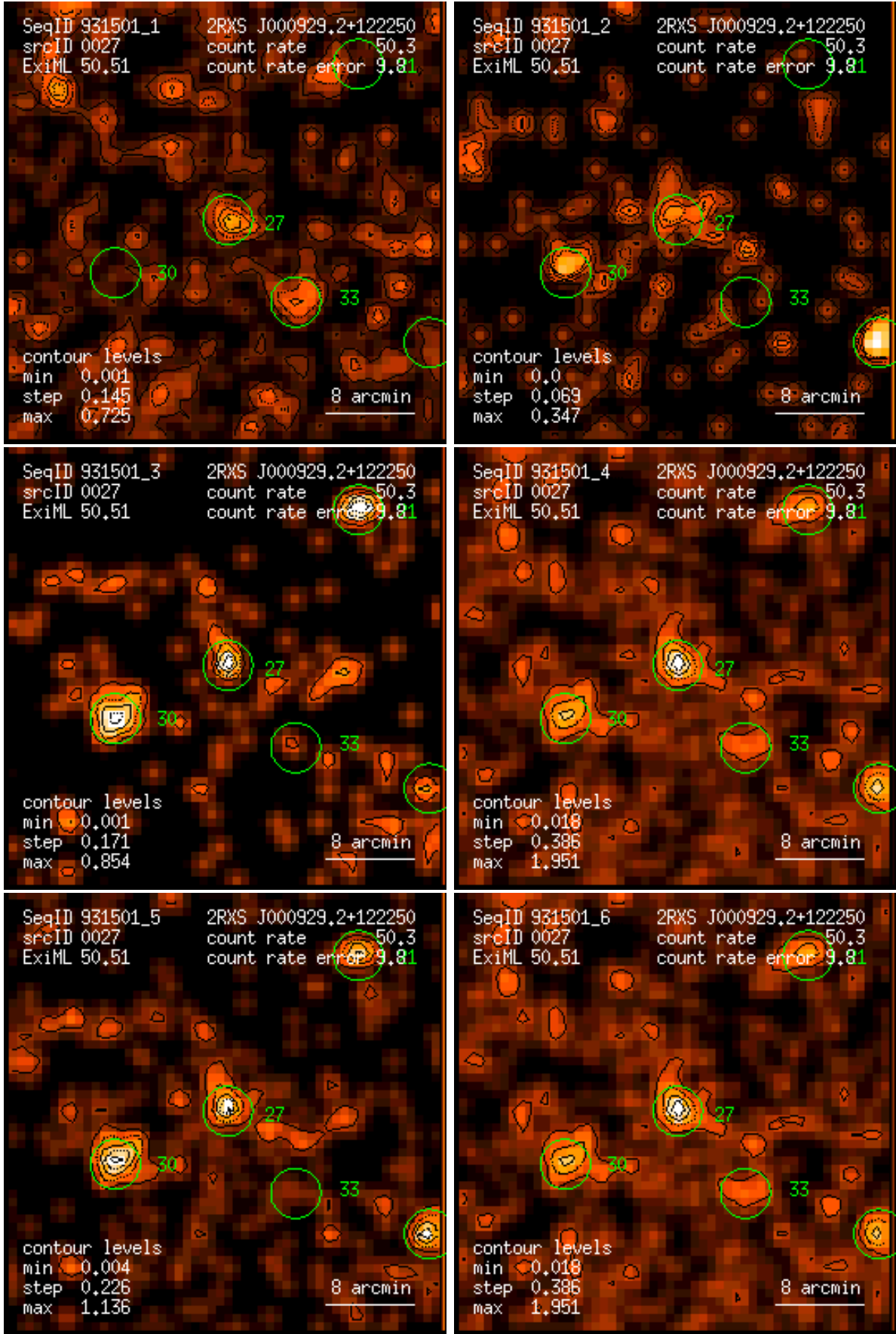
Figure 27: RASS 931501: detection 0027: band rate images, Gaussian filter: (1) PSPC channels 11 – 41, (2) 52 – 90, (3) 91 – 201, (4) 11 – 235, (5) 52 – 201, (6) 11 – 201. Broad band rates in counts/ks. Band rate contour levels in counts/ks/arcmin 2 .
