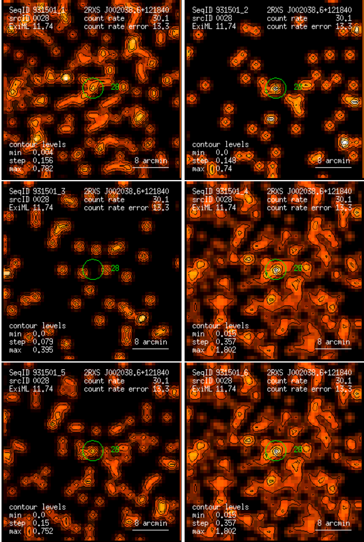
Figure 28: RASS 931501: detection 0028: band rate images, Gaussian filter: (1) PSPC channels 11 – 41, (2) 52 – 90, (3) 91 – 201, (4) 11 – 235, (5) 52 – 201, (6) 11 – 201. Broad band rates in counts/ks. Band rate contour levels in counts/ks/arcmin 2 .
