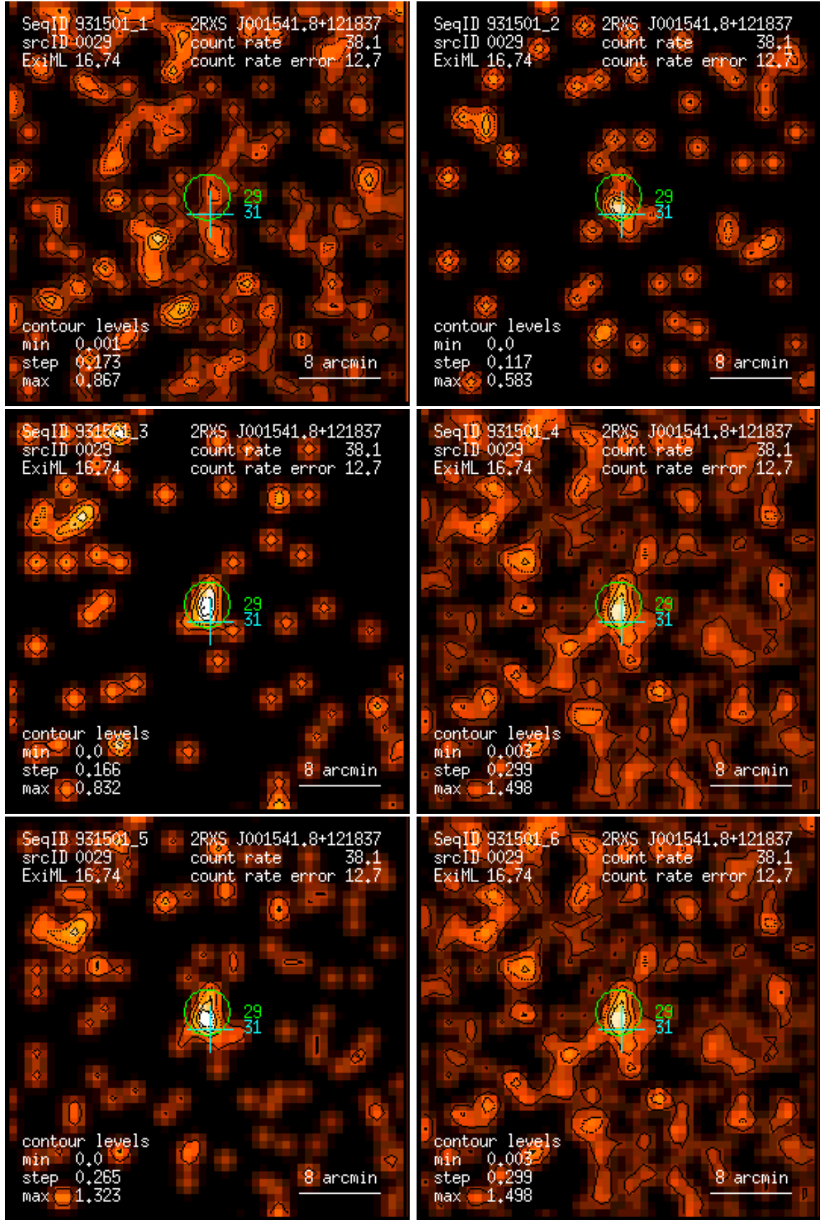
Figure 29: RASS 931501: detection 0029: band rate images, Gaussian filter: (1) PSPC channels 11 – 41, (2) 52 – 90, (3) 91 – 201, (4) 11 – 235, (5) 52 – 201, (6) 11 – 201. Broad band rates in counts/ks. Band rate contour levels in counts/ks/arcmin 2 .
