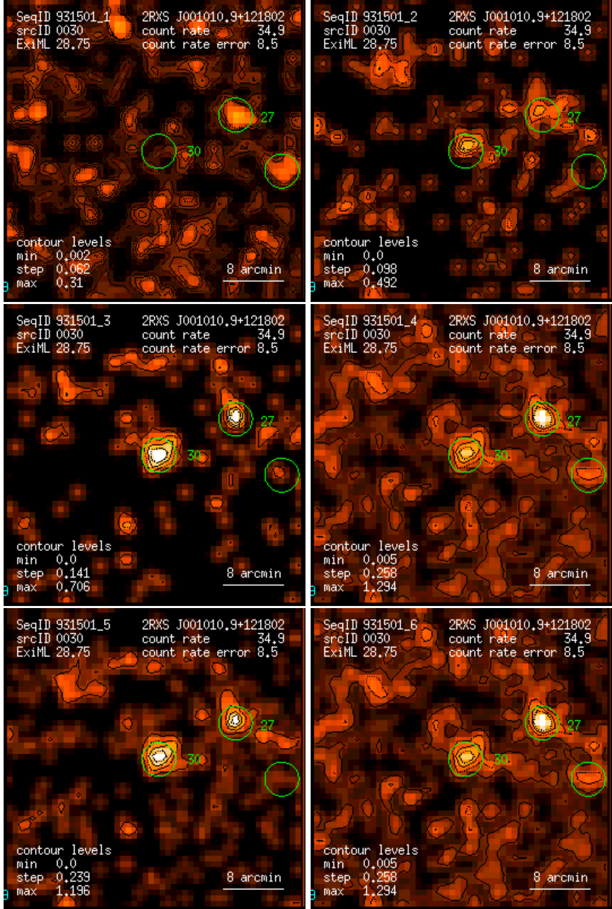
Figure 30: RASS 931501: detection 0030: band rate images, Gaussian filter: (1) PSPC channels 11 – 41, (2) 52 – 90, (3) 91 – 201, (4) 11 – 235, (5) 52 – 201, (6) 11 – 201. Broad band rates in counts/ks. Band rate contour levels in counts/ks/arcmin 2 .
