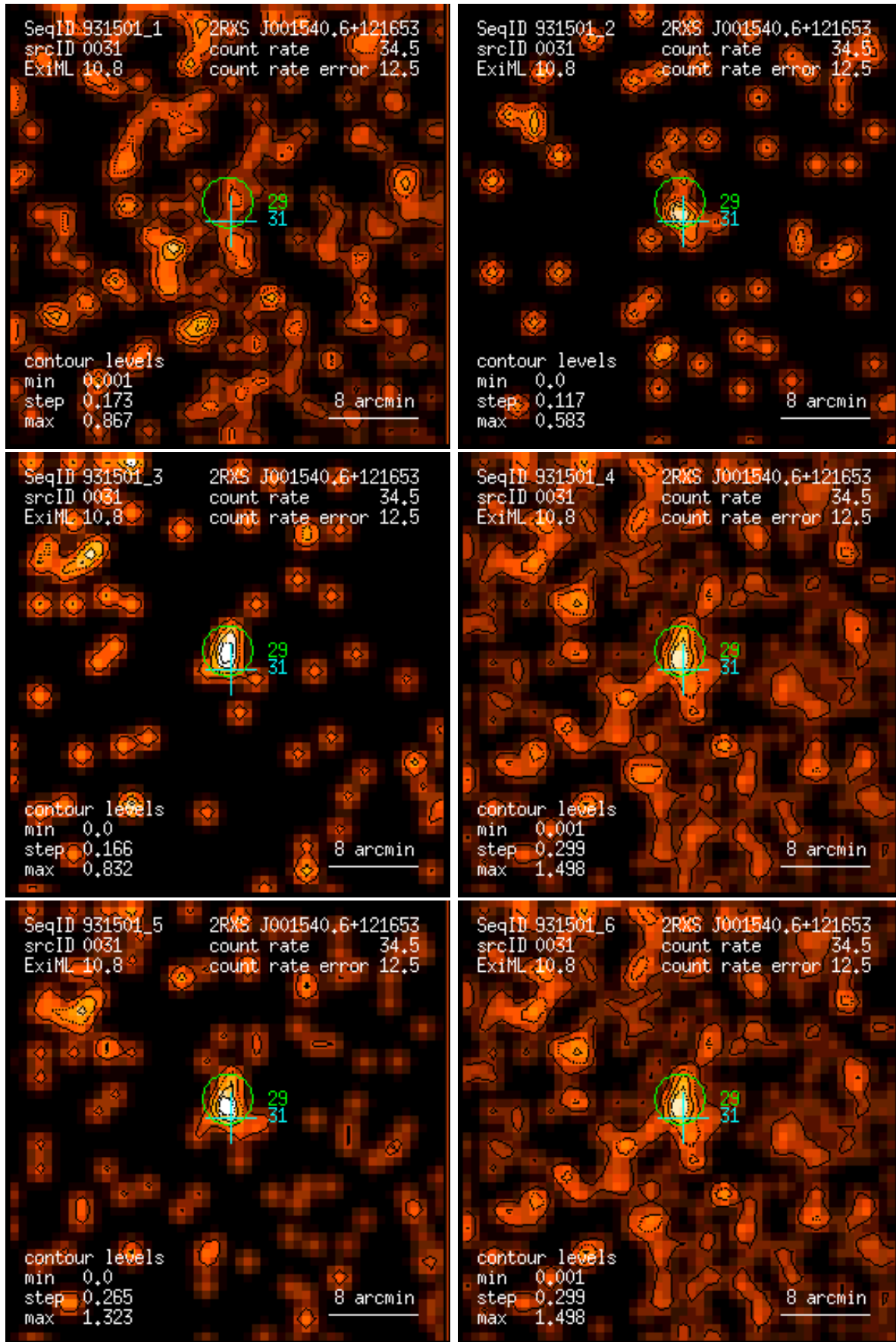
Figure 31: RASS 931501: detection 0031: band rate images, Gaussian filter: (1) PSPC channels 11 – 41, (2) 52 – 90, (3) 91 – 201, (4) 11 – 235, (5) 52 – 201, (6) 11 – 201. Broad band rates in counts/ks. Band rate contour levels in counts/ks/arcmin 2 .
