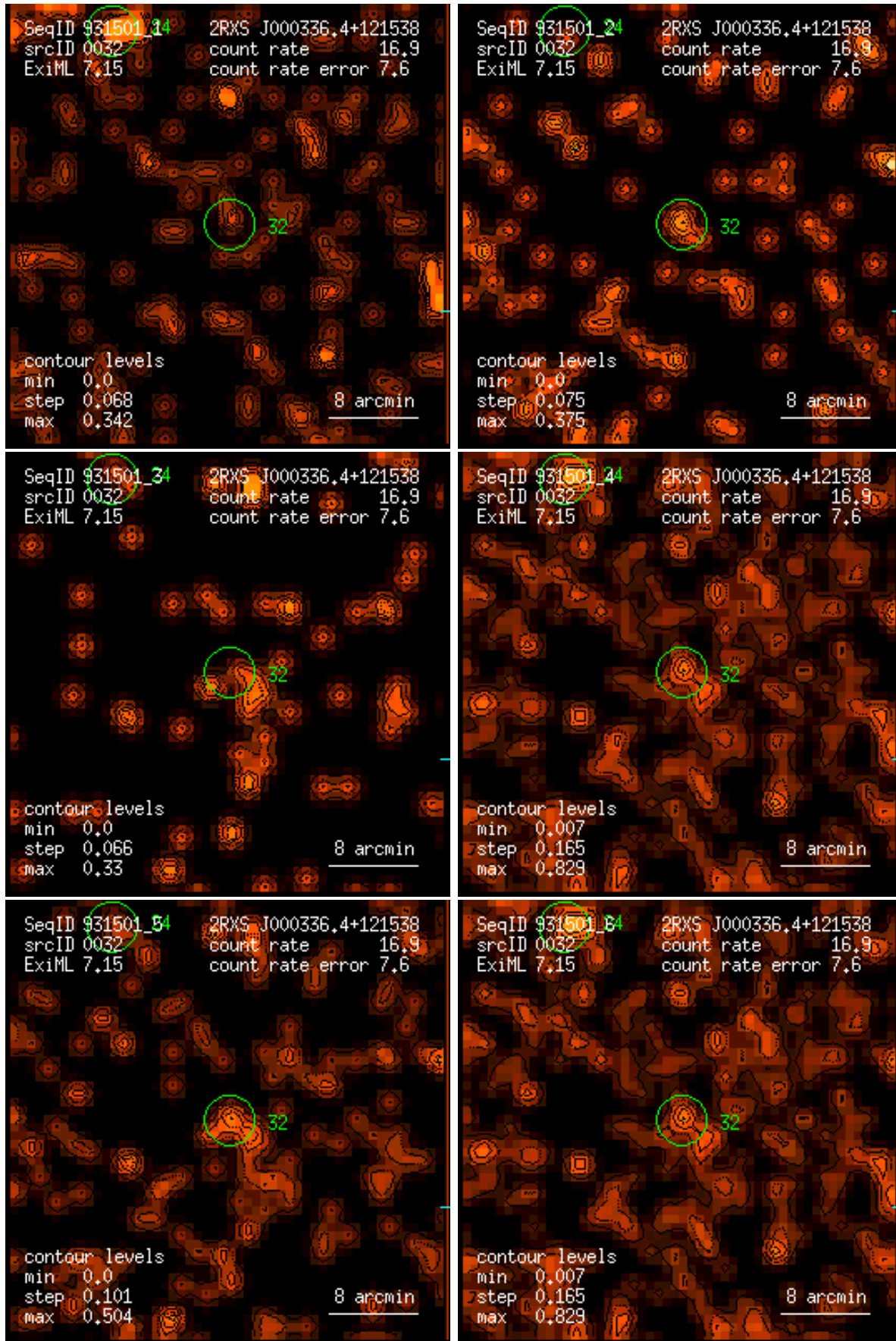
Figure 32: RASS 931501: detection 0032: band rate images, Gaussian filter: (1) PSPC channels 11 – 41, (2) 52 – 90, (3) 91 – 201, (4) 11 – 235, (5) 52 – 201, (6) 11 – 201. Broad band rates in counts/ks. Band rate contour levels in counts/ks/arcmin 2 .
