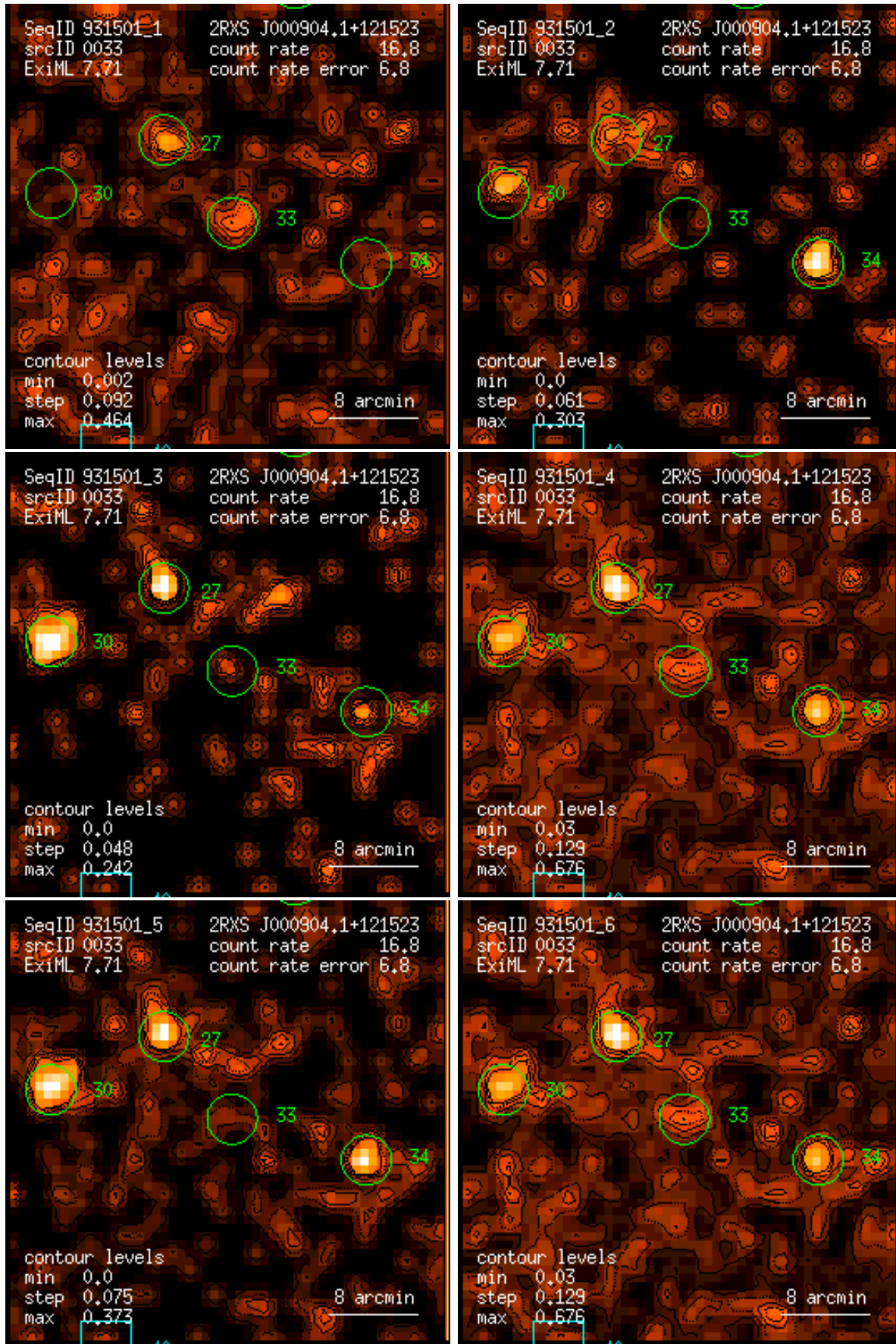
Figure 33: RASS 931501: detection 0033: band rate images, Gaussian filter: (1) PSPC channels 11 – 41, (2) 52 – 90, (3) 91 – 201, (4) 11 – 235, (5) 52 – 201, (6) 11 – 201. Broad band rates in counts/ks. Band rate contour levels in counts/ks/arcmin 2 .
