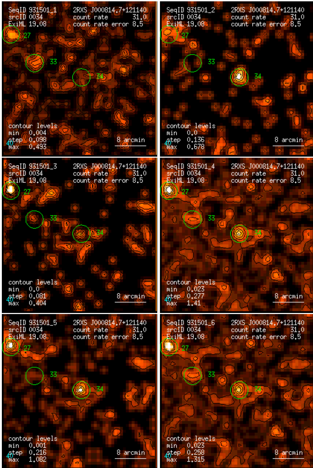
Figure 34: RASS 931501: detection 0034: band rate images, Gaussian filter: (1) PSPC channels 11 – 41, (2) 52 – 90, (3) 91 – 201, (4) 11 – 235, (5) 52 – 201, (6) 11 – 201. Broad band rates in counts/ks. Band rate contour levels in counts/ks/arcmin 2 .
