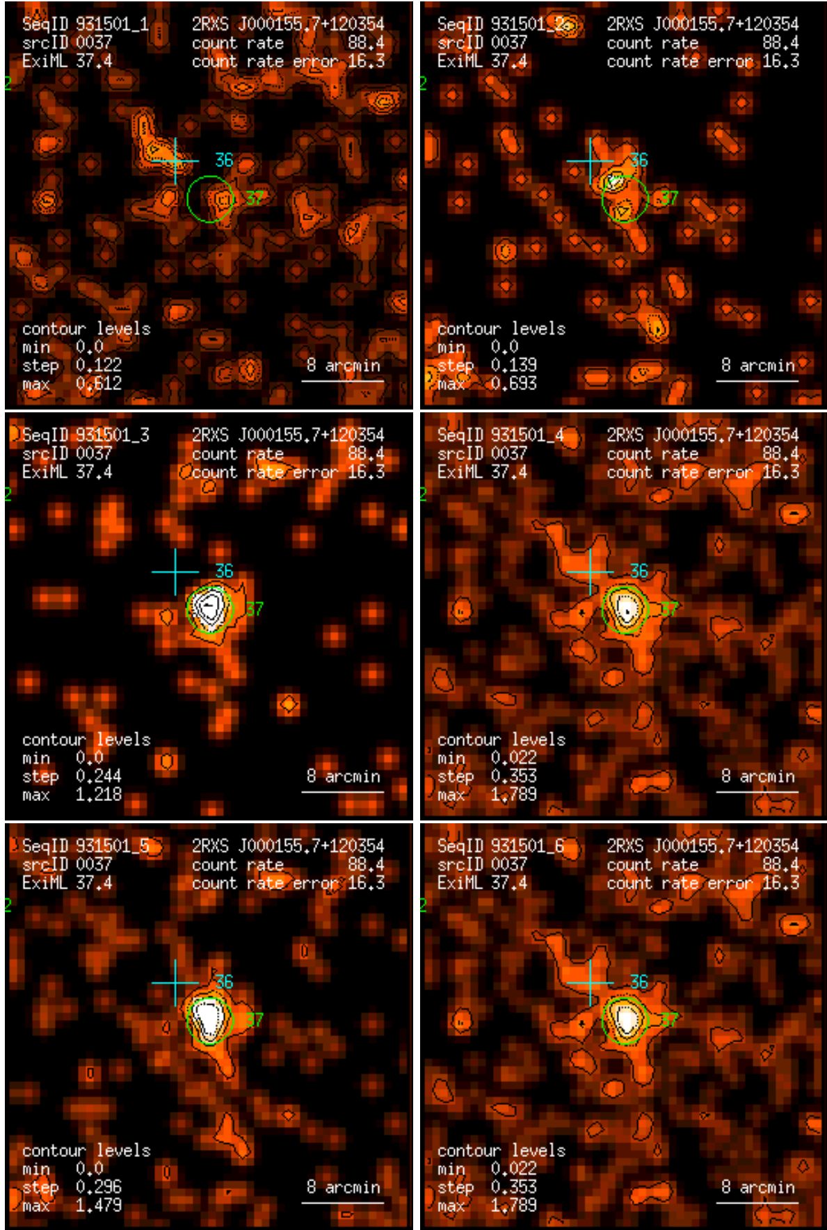
Figure 37: RASS 931501: detection 0037: band rate images, Gaussian filter: (1) PSPC channels 11 – 41, (2) 52 – 90, (3) 91 – 201, (4) 11 – 235, (5) 52 – 201, (6) 11 – 201. Broad band rates in counts/ks. Band rate contour levels in counts/ks/arcmin 2 .
