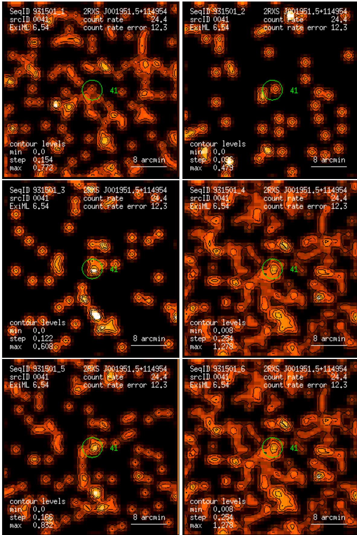
Figure 41: RASS 931501: detection 0041: band rate images, Gaussian filter: (1) PSPC channels 11 – 41, (2) 52 – 90, (3) 91 – 201, (4) 11 – 235, (5) 52 – 201, (6) 11 – 201. Broad band rates in counts/ks. Band rate contour levels in counts/ks/arcmin 2 .
