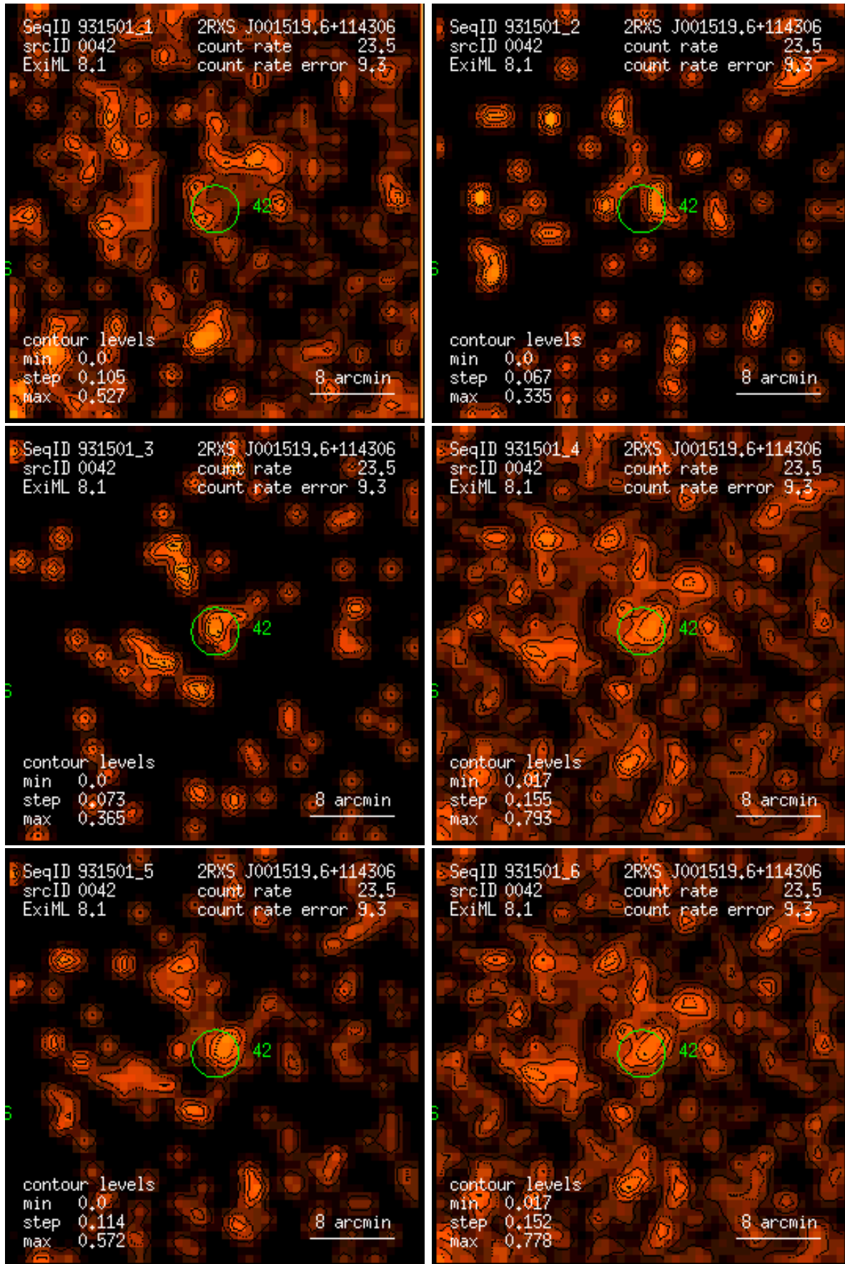
Figure 42: RASS 931501: detection 0042: band rate images, Gaussian filter: (1) PSPC channels 11 – 41, (2) 52 – 90, (3) 91 – 201, (4) 11 – 235, (5) 52 – 201, (6) 11 – 201. Broad band rates in counts/ks. Band rate contour levels in counts/ks/arcmin 2 .
