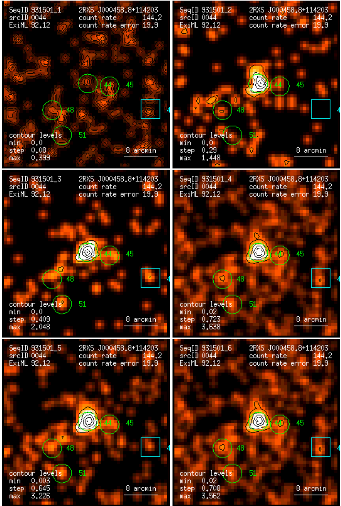
Figure 44: RASS 931501: detection 0044: band rate images, Gaussian filter: (1) PSPC channels 11 – 41, (2) 52 – 90, (3) 91 – 201, (4) 11 – 235, (5) 52 – 201, (6) 11 – 201. Broad band rates in counts/ks. Band rate contour levels in counts/ks/arcmin 2 .
