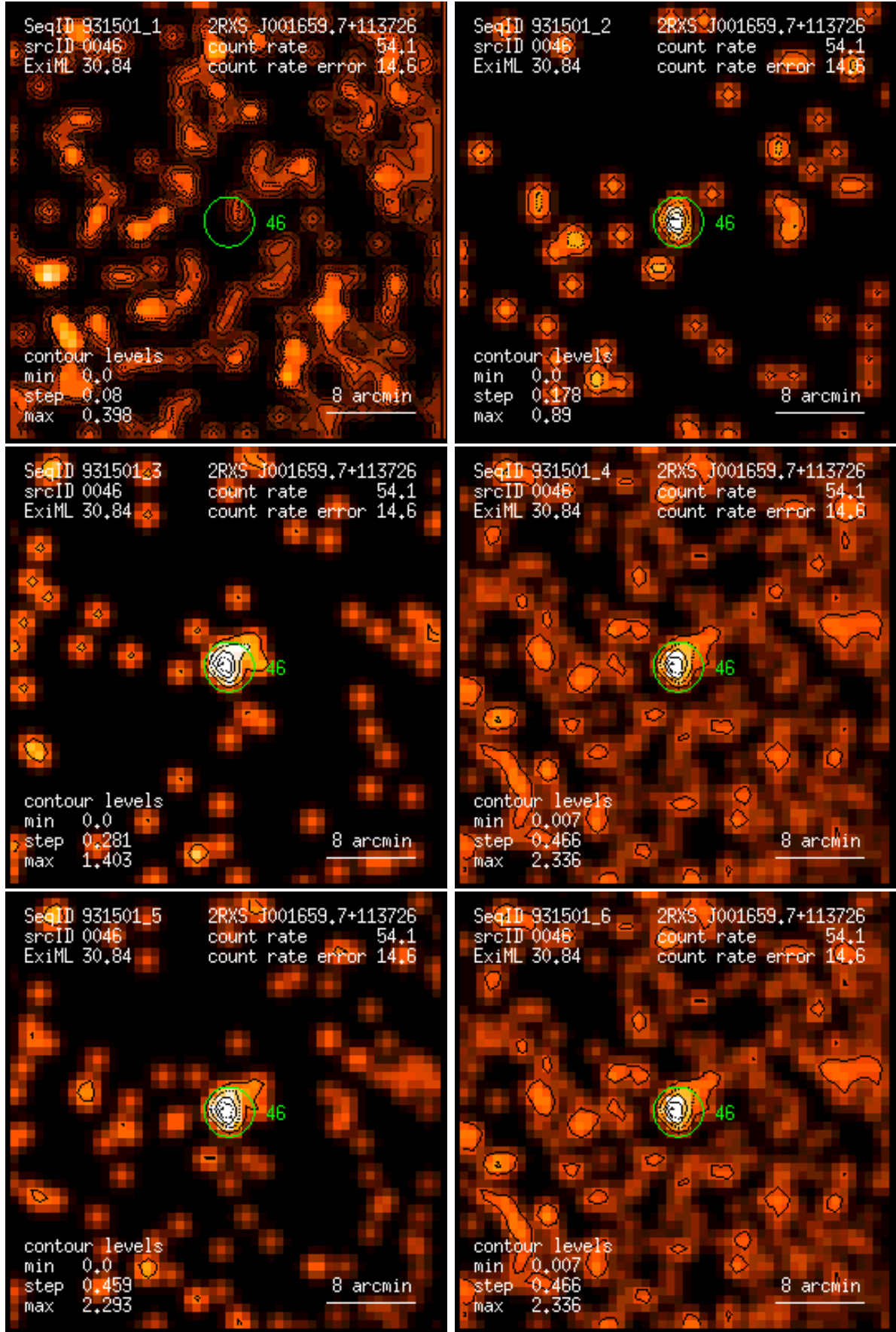
Figure 46: RASS 931501: detection 0046: band rate images, Gaussian filter: (1) PSPC channels 11 – 41, (2) 52 – 90, (3) 91 – 201, (4) 11 – 235, (5) 52 – 201, (6) 11 – 201. Broad band rates in counts/ks. Band rate contour levels in counts/ks/arcmin 2 .
