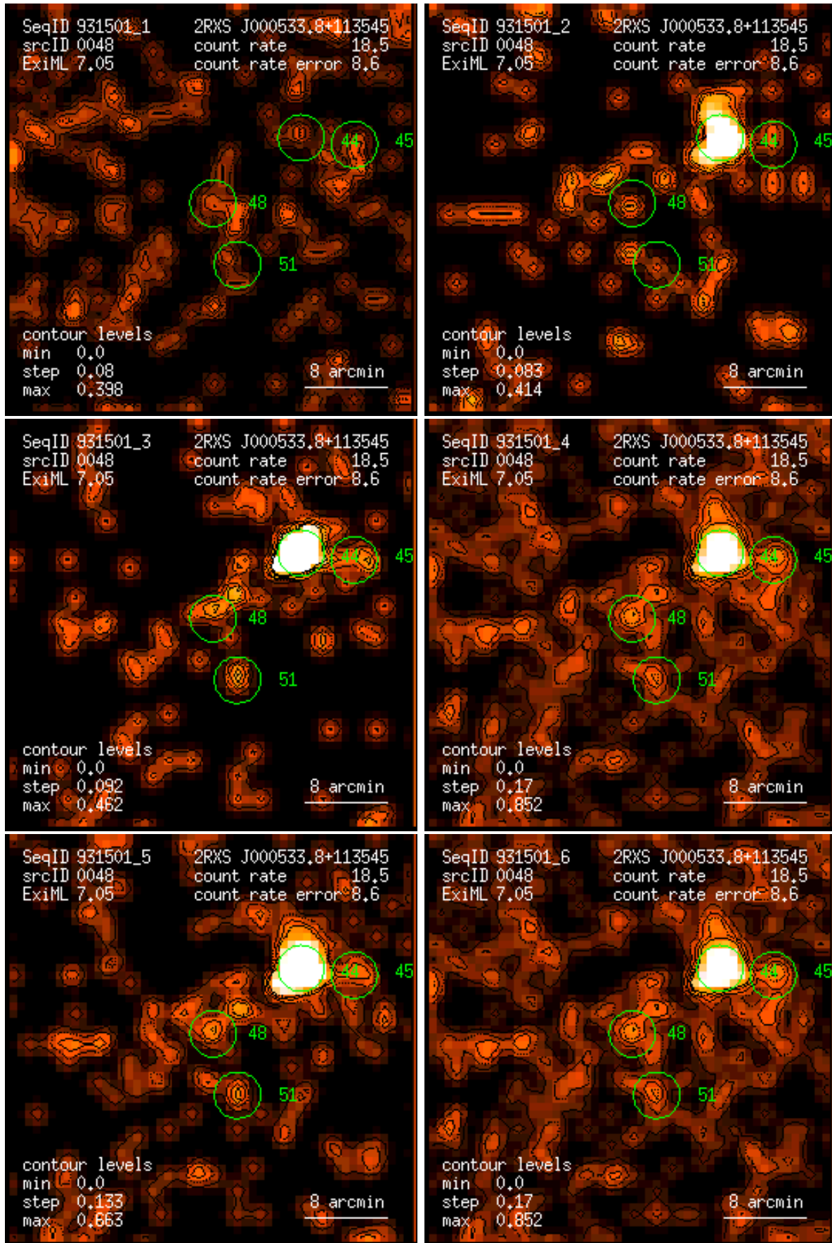
Figure 48: RASS 931501: detection 0048: band rate images, Gaussian filter: (1) PSPC channels 11 – 41, (2) 52 – 90, (3) 91 – 201, (4) 11 – 235, (5) 52 – 201, (6) 11 – 201. Broad band rates in counts/ks. Band rate contour levels in counts/ks/arcmin 2 .
