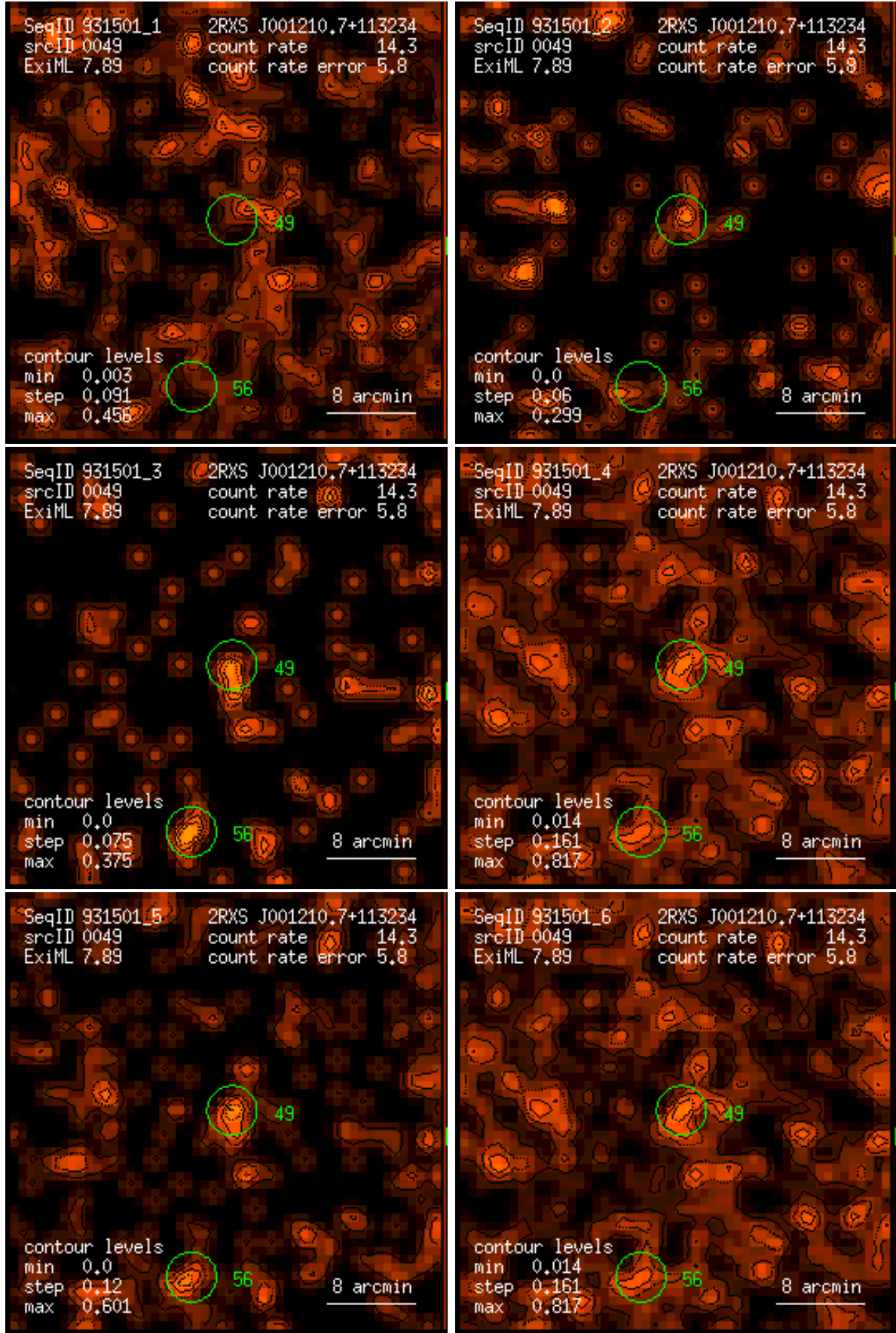
Figure 49: RASS 931501: detection 0049: band rate images, Gaussian filter: (1) PSPC channels 11 – 41, (2) 52 – 90, (3) 91 – 201, (4) 11 – 235, (5) 52 – 201, (6) 11 – 201. Broad band rates in counts/ks. Band rate contour levels in counts/ks/arcmin 2 .
