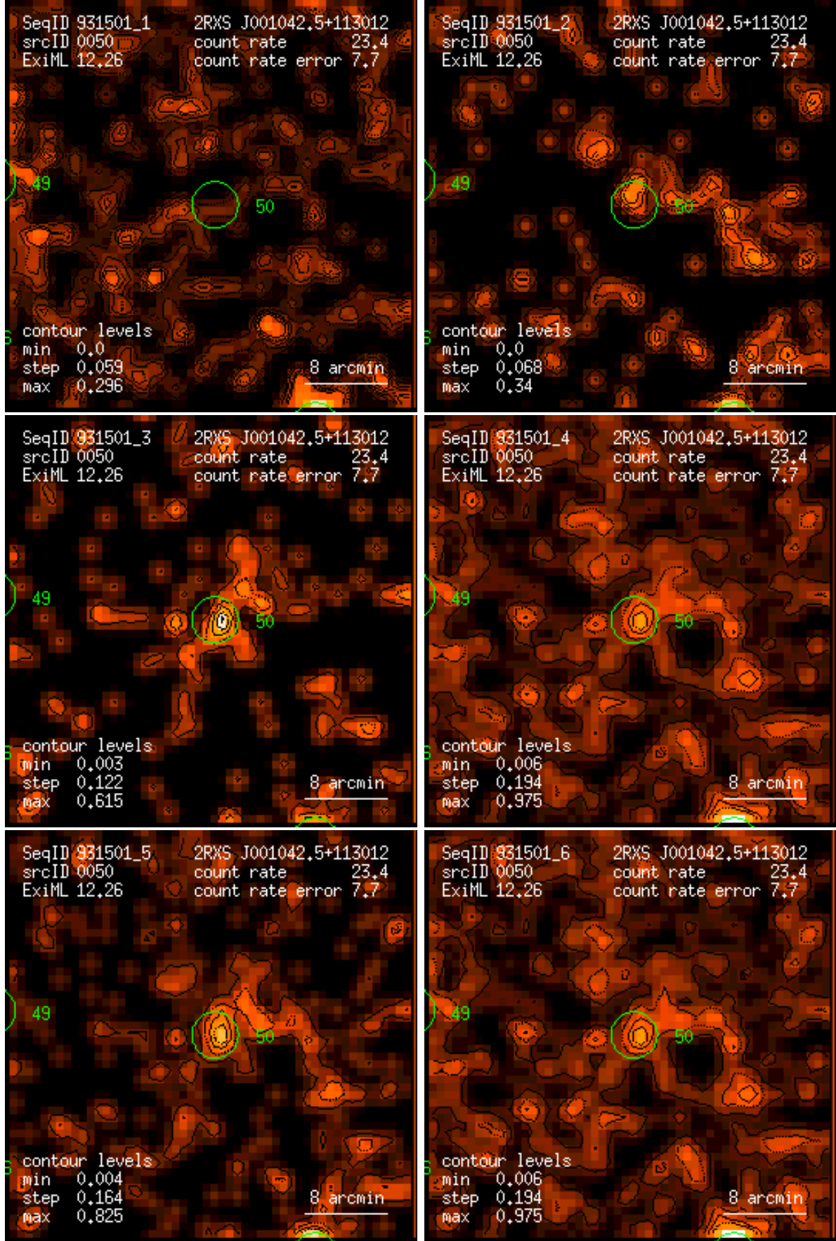
Figure 50: RASS 931501: detection 0050: band rate images, Gaussian filter: (1) PSPC channels 11 – 41, (2) 52 – 90, (3) 91 – 201, (4) 11 – 235, (5) 52 – 201, (6) 11 – 201. Broad band rates in counts/ks. Band rate contour levels in counts/ks/arcmin 2 .
