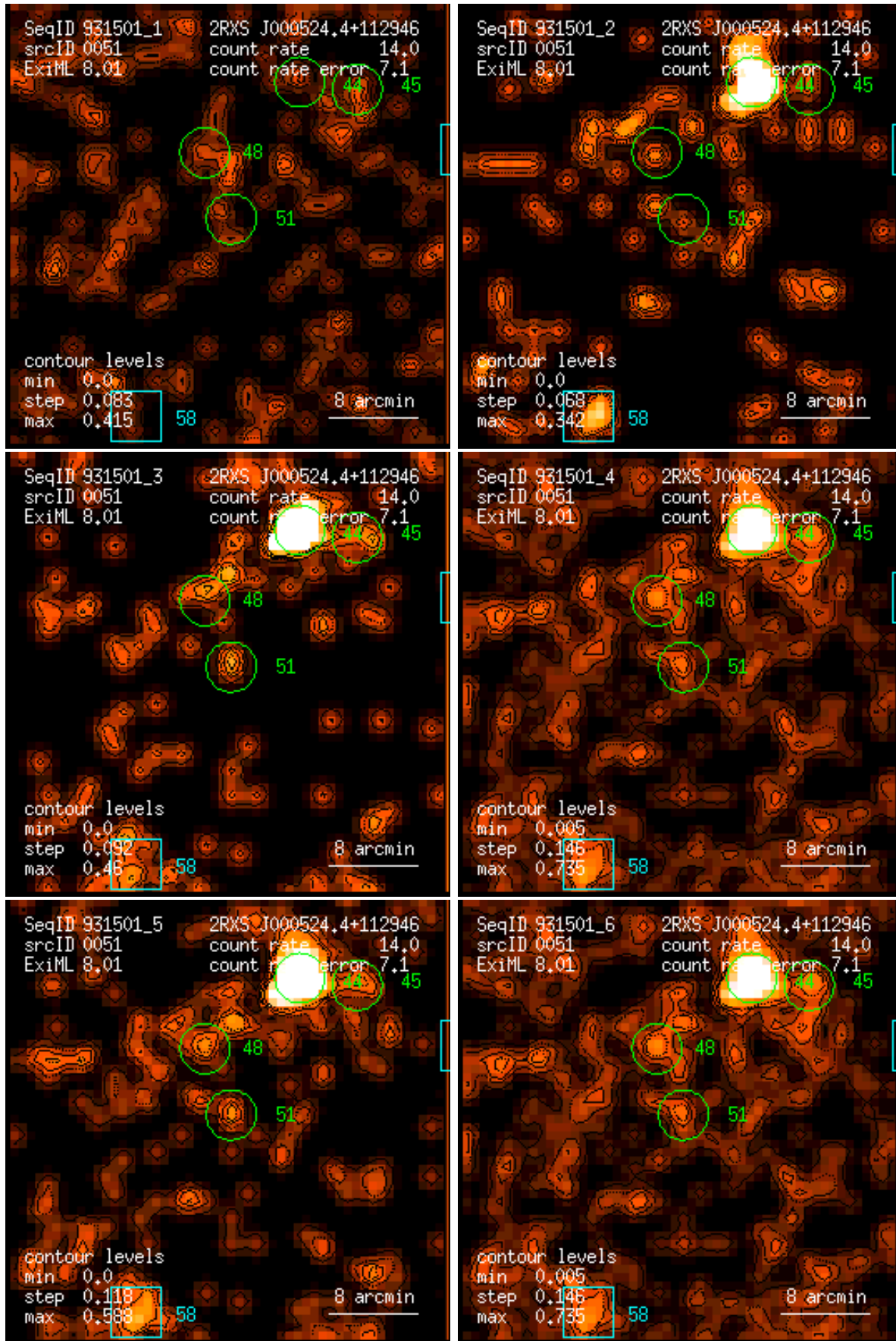
Figure 51: RASS 931501: detection 0051: band rate images, Gaussian filter: (1) PSPC channels 11 – 41, (2) 52 – 90, (3) 91 – 201, (4) 11 – 235, (5) 52 – 201, (6) 11 – 201. Broad band rates in counts/ks. Band rate contour levels in counts/ks/arcmin 2 .
