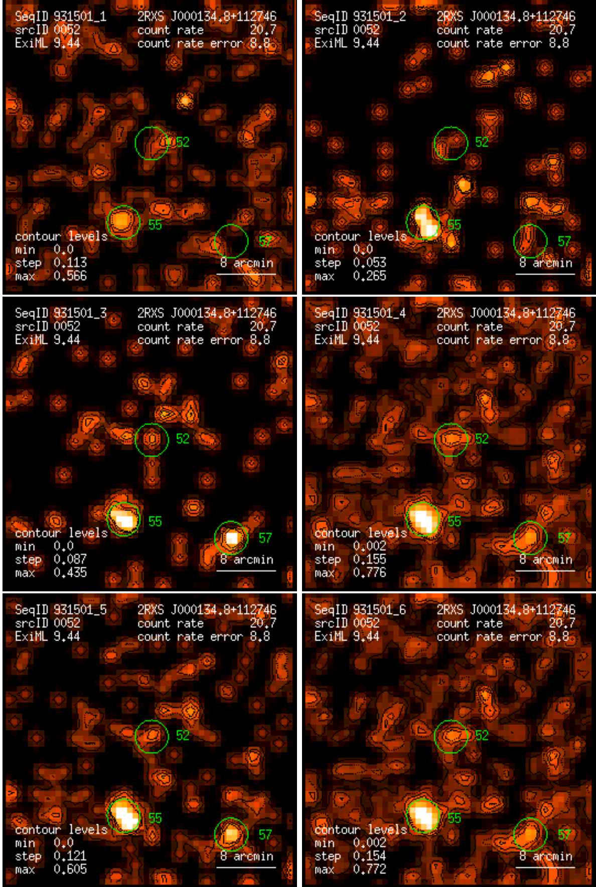
Figure 52: RASS 931501: detection 0052: band rate images, Gaussian filter: (1) PSPC channels 11 – 41, (2) 52 – 90, (3) 91 – 201, (4) 11 – 235, (5) 52 – 201, (6) 11 – 201. Broad band rates in counts/ks. Band rate contour levels in counts/ks/arcmin 2 .
