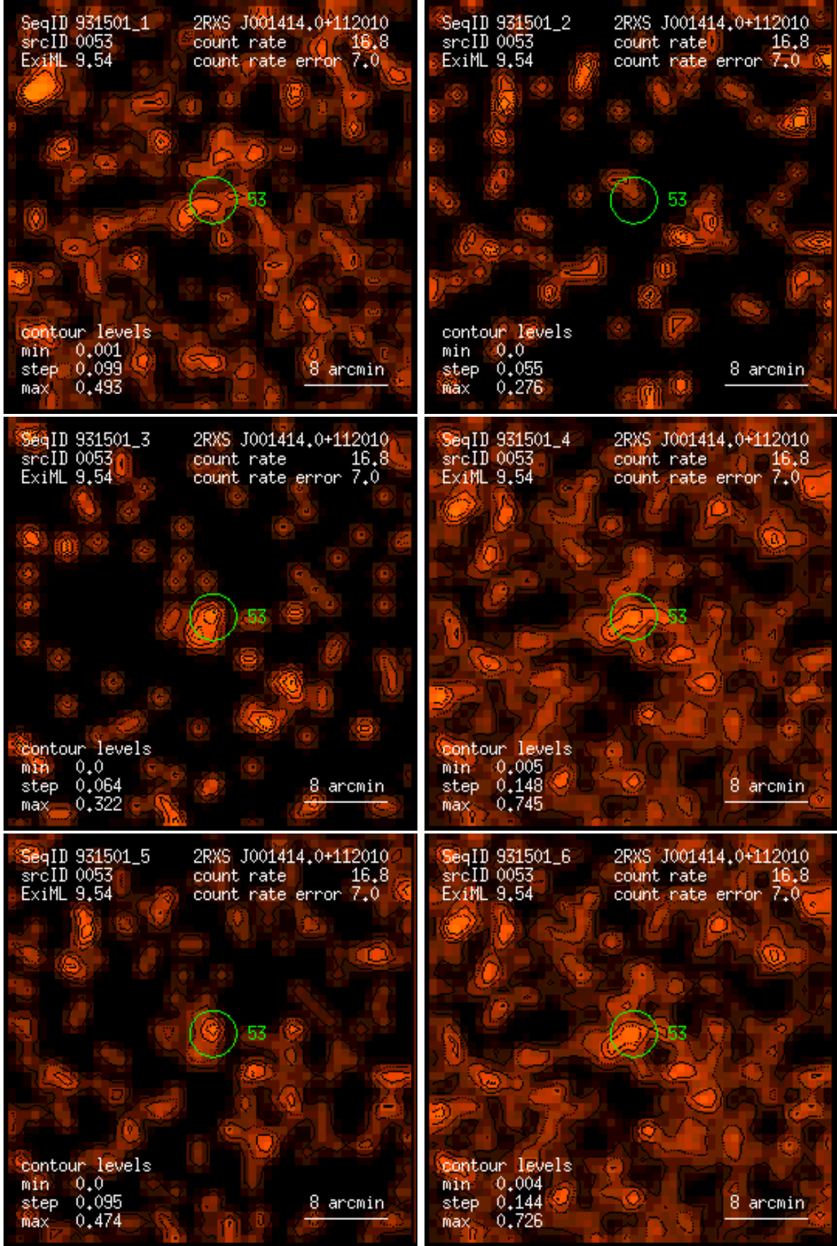
Figure 53: RASS 931501: detection 0053: band rate images, Gaussian filter: (1) PSPC channels 11 – 41, (2) 52 – 90, (3) 91 – 201, (4) 11 – 235, (5) 52 – 201, (6) 11 – 201. Broad band rates in counts/ks. Band rate contour levels in counts/ks/arcmin 2 .
