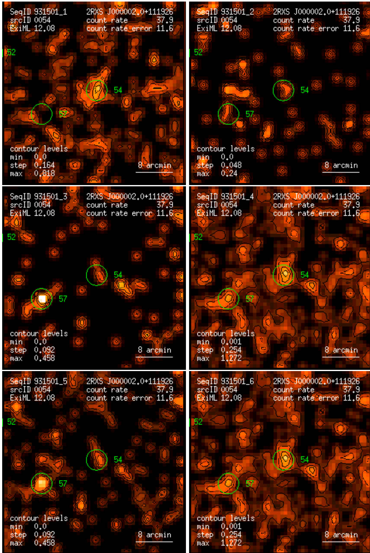
Figure 54: RASS 931501: detection 0054: band rate images, Gaussian filter: (1) PSPC channels 11 – 41, (2) 52 – 90, (3) 91 – 201, (4) 11 – 235, (5) 52 – 201, (6) 11 – 201. Broad band rates in counts/ks. Band rate contour levels in counts/ks/arcmin 2 .
