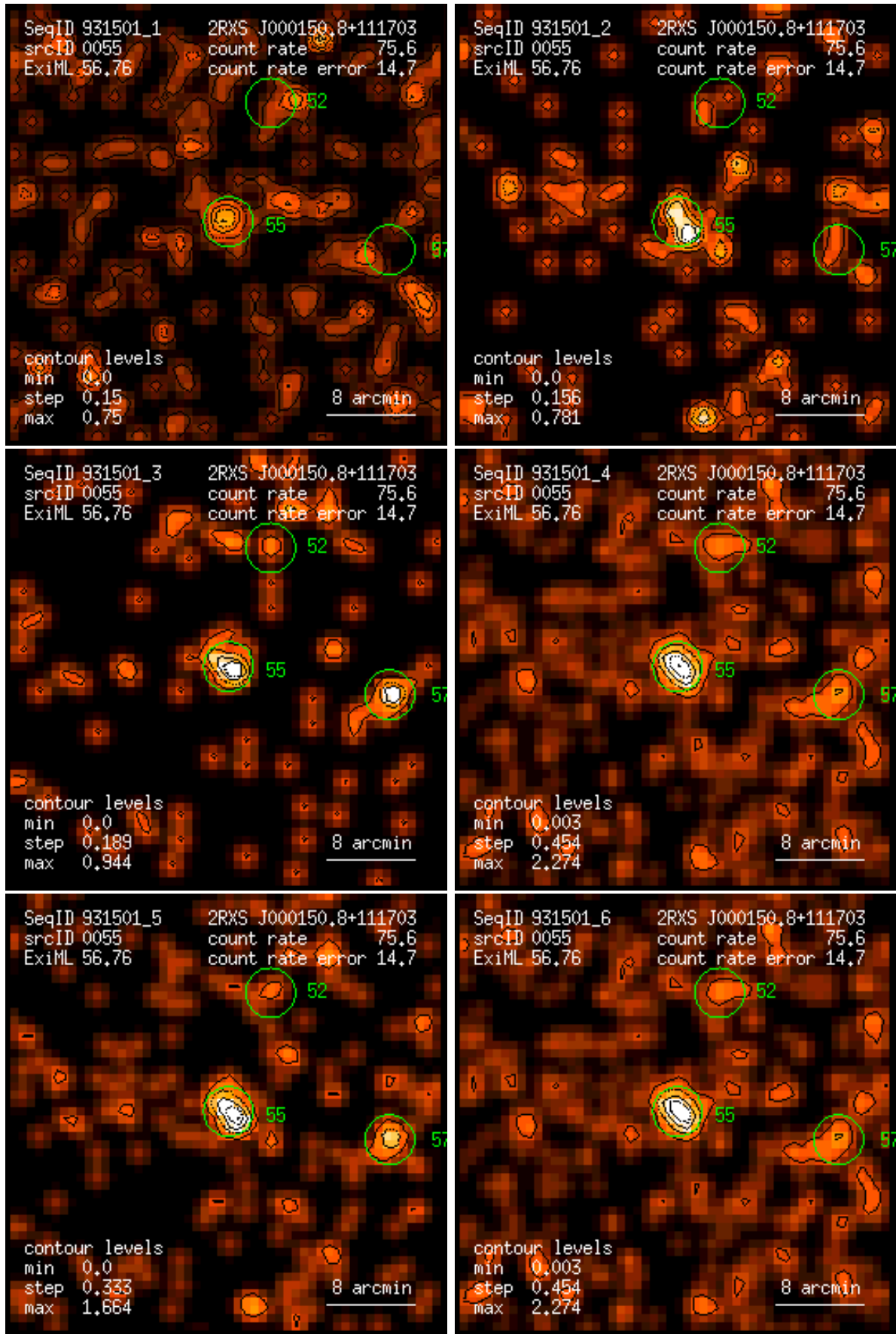
Figure 55: RASS 931501: detection 0055: band rate images, Gaussian filter: (1) PSPC channels 11 – 41, (2) 52 – 90, (3) 91 – 201, (4) 11 – 235, (5) 52 – 201, (6) 11 – 201. Broad band rates in counts/ks. Band rate contour levels in counts/ks/arcmin 2 .
