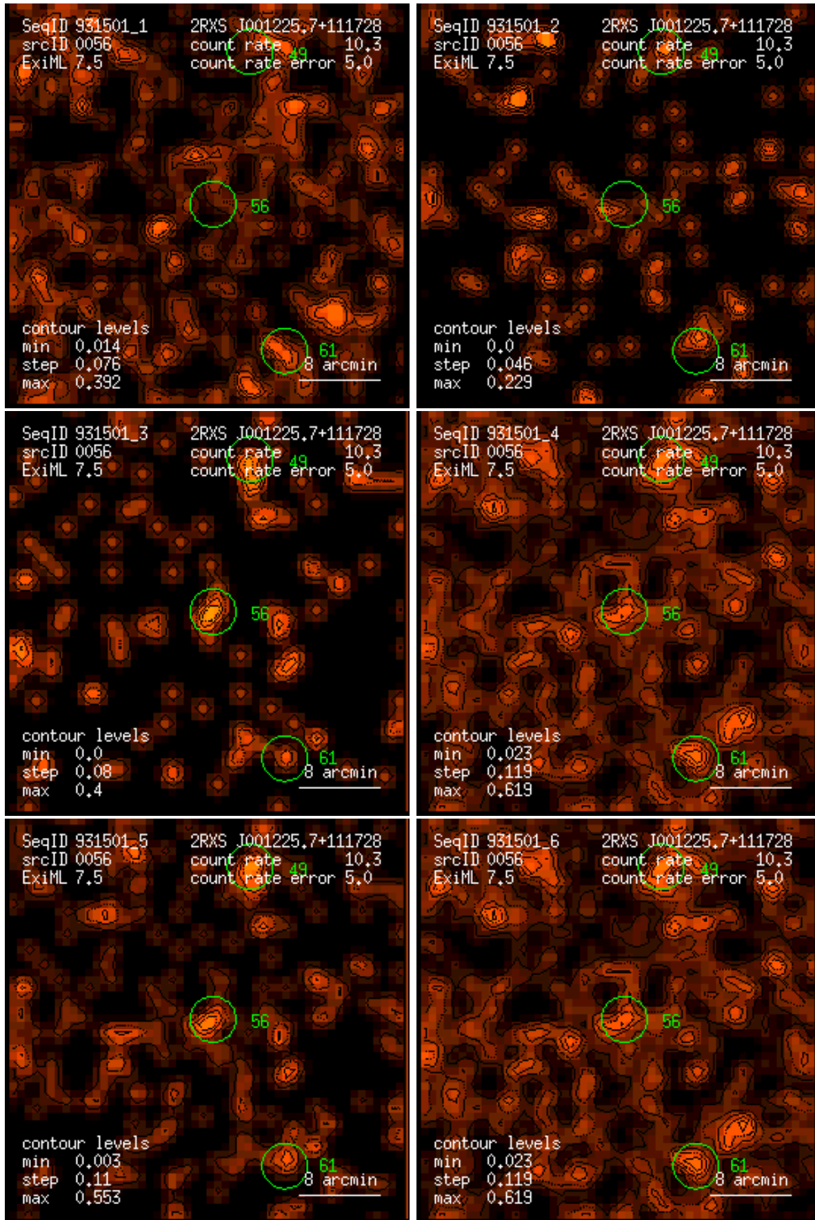
Figure 56: RASS 931501: detection 0056: band rate images, Gaussian filter: (1) PSPC channels 11 – 41, (2) 52 – 90, (3) 91 – 201, (4) 11 – 235, (5) 52 – 201, (6) 11 – 201. Broad band rates in counts/ks. Band rate contour levels in counts/ks/arcmin 2 .
