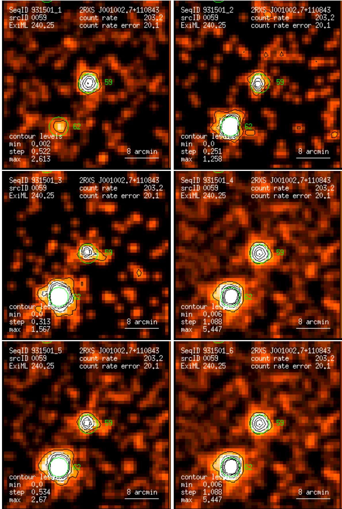
Figure 59: RASS 931501: detection 0059: band rate images, Gaussian filter: (1) PSPC channels 11 – 41, (2) 52 – 90, (3) 91 – 201, (4) 11 – 235, (5) 52 – 201, (6) 11 – 201. Broad band rates in counts/ks. Band rate contour levels in counts/ks/arcmin 2 .
