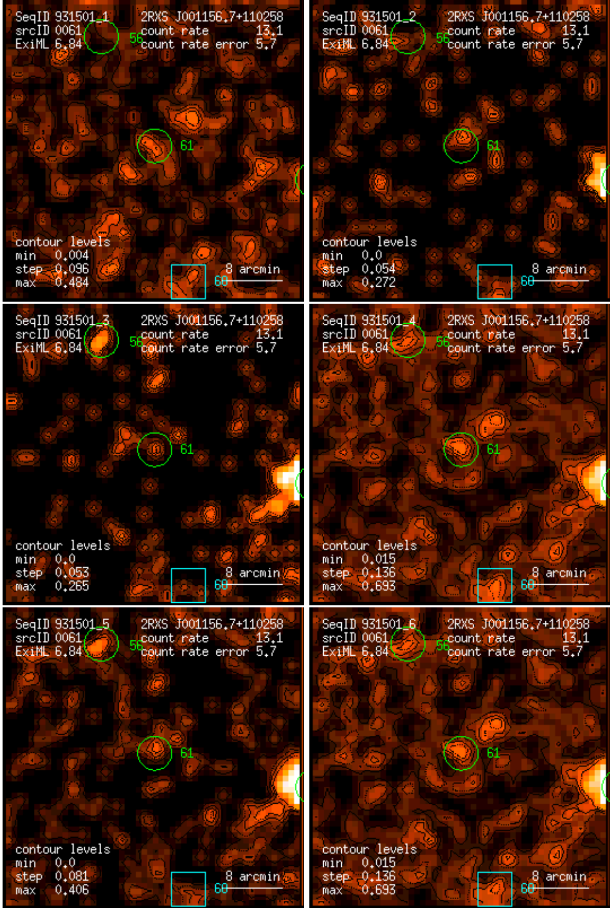
Figure 61: RASS 931501: detection 0061: band rate images, Gaussian filter: (1) PSPC channels 11 – 41, (2) 52 – 90, (3) 91 – 201, (4) 11 – 235, (5) 52 – 201, (6) 11 – 201. Broad band rates in counts/ks. Band rate contour levels in counts/ks/arcmin 2 .
